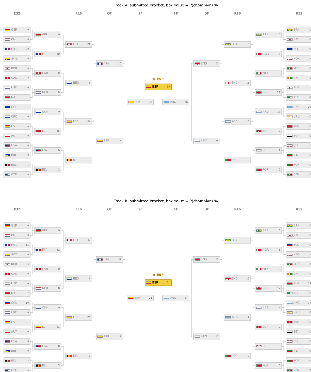
Figure 19: The submitted bracket re-valued by champion probability under Track A (top) and Track B (bottom) at live edition M072; the gold box is each track's most likely champion and greyed boxes are teams eliminated by confirmed results. The locked submitted bracket is Figure 18.
