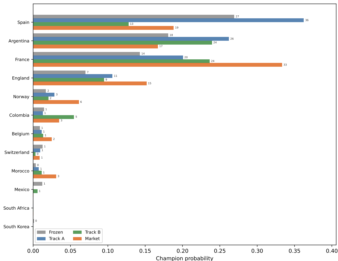
Figure 4: Champion probability, four ways: Frozen / Track A / Track B / Market, top twelve teams (live edition M072)
