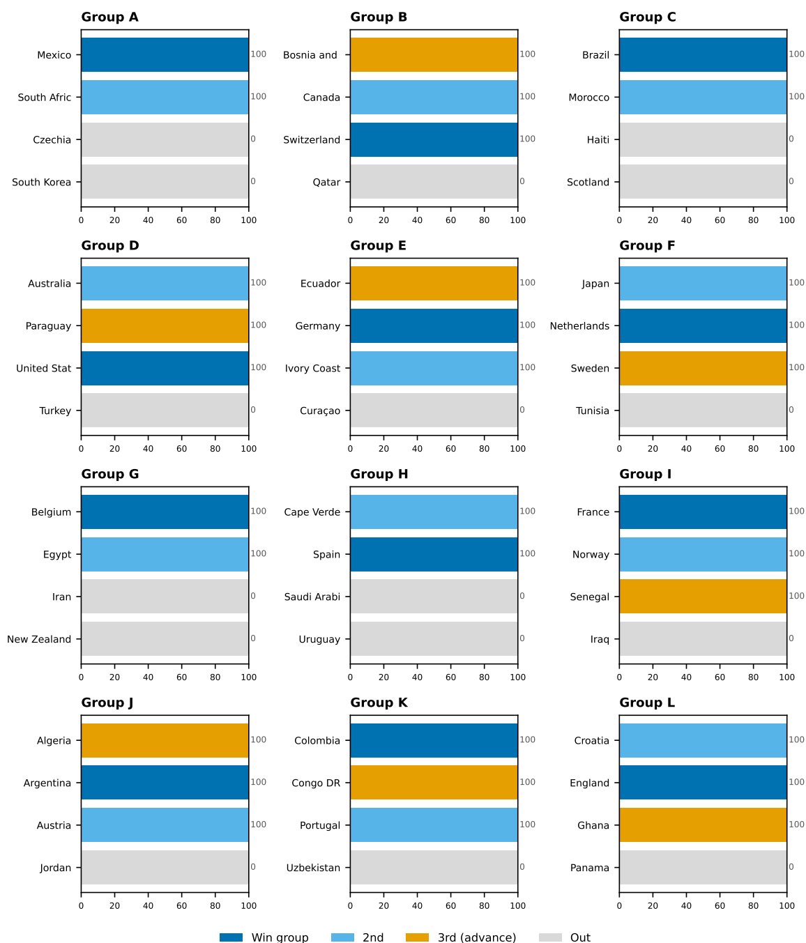
Figure 17: Qualification probability by team — Track B (result-conditioning + live Elo + bookmaker odds; live edition M072)
