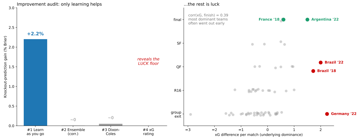
Figure 16: Candidate improvements tested on 2018 and 2022
