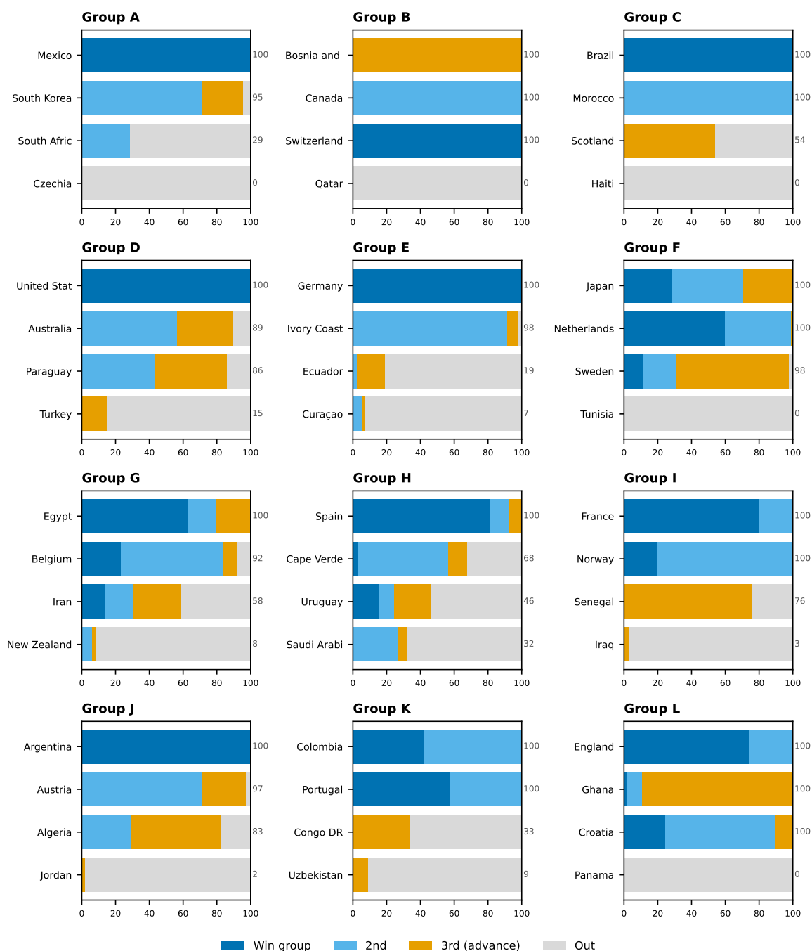
Figure 16: Qualification probability by team — Track A (conditioned on 53 results, June 10 ratings frozen; live edition M053)
