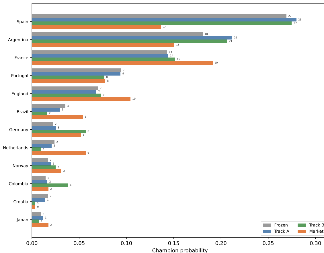
Figure 4: Champion probability, four ways: Frozen / Track A / Track B / Market, top twelve teams (live edition M053)
