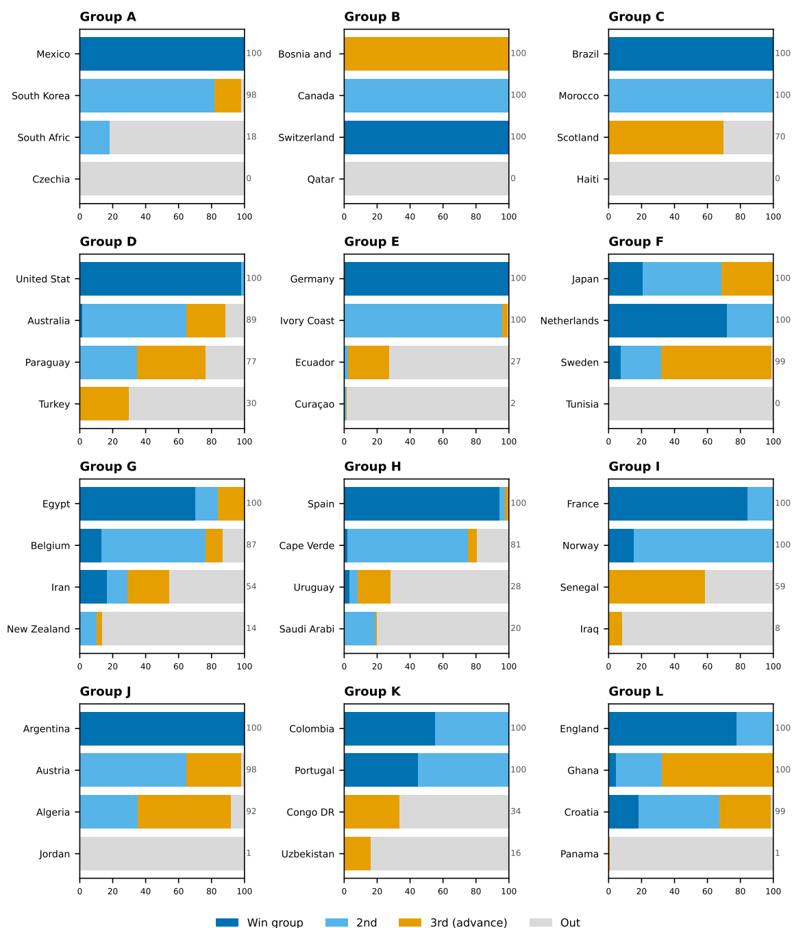
Figure 17: Qualification probability by team — Track B (result-conditioning + live Elo + bookmaker odds; live edition M053)
