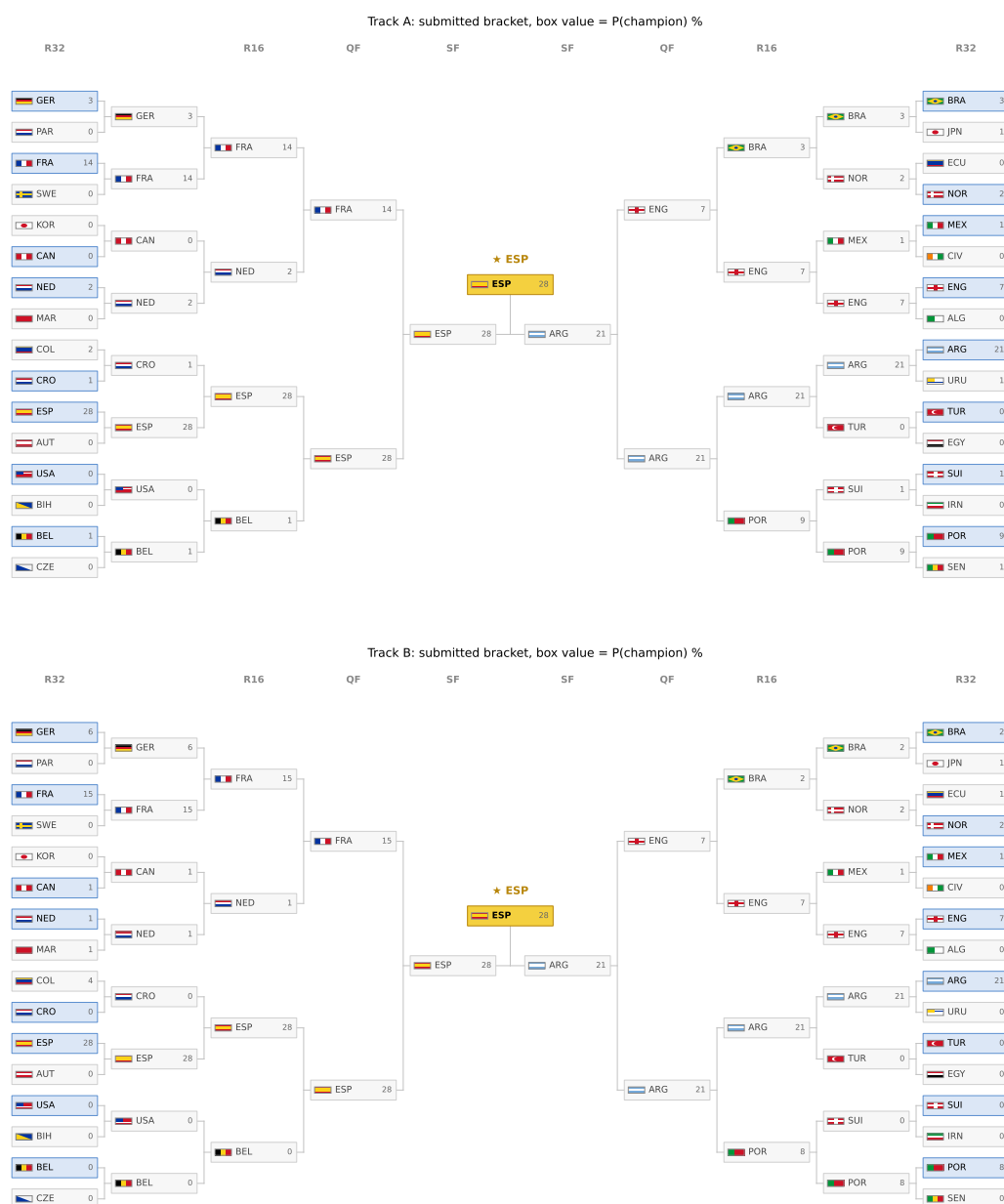
Figure 19: The submitted bracket re-valued by champion probability under Track A (top) and Track B (bottom) at live edition M053; the gold box is each track's most likely champion and greyed boxes are teams eliminated by confirmed results. The locked submitted bracket is Figure 18.
