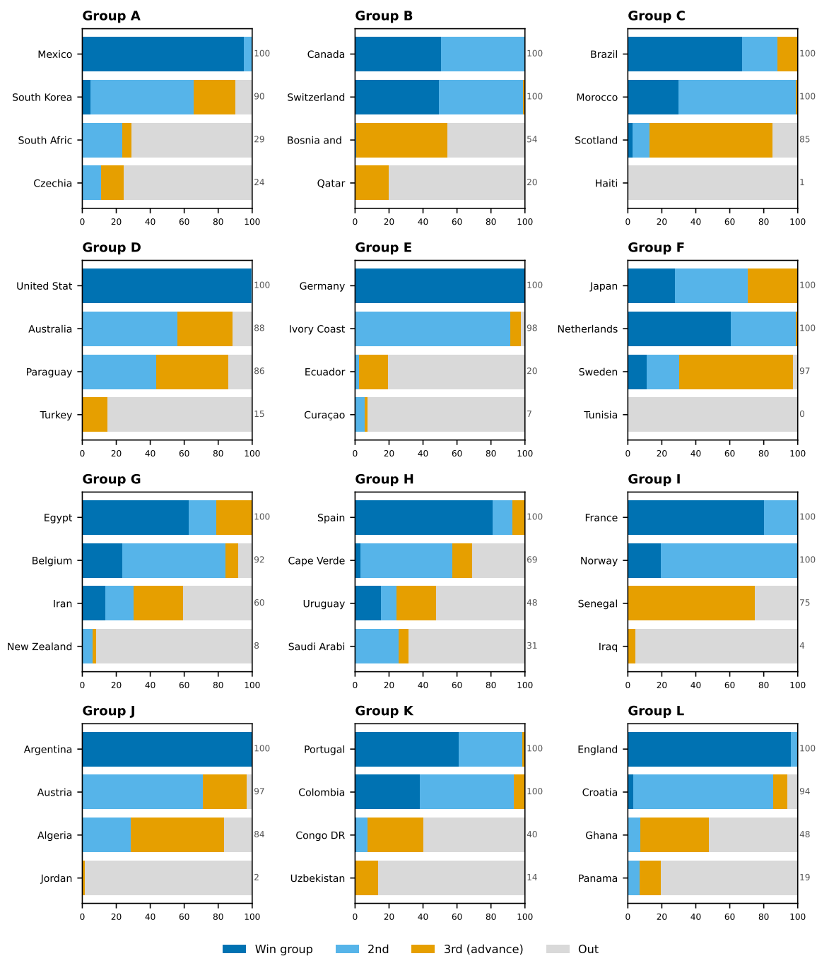
Figure 16: Qualification probability by team — Track A (conditioned on 45 results, June 10 ratings frozen; live edition M047)
