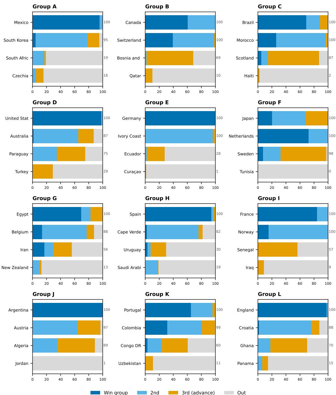
Figure 17: Qualification probability by team — Track B (result-conditioning + live Elo + bookmaker odds; live edition M047)
