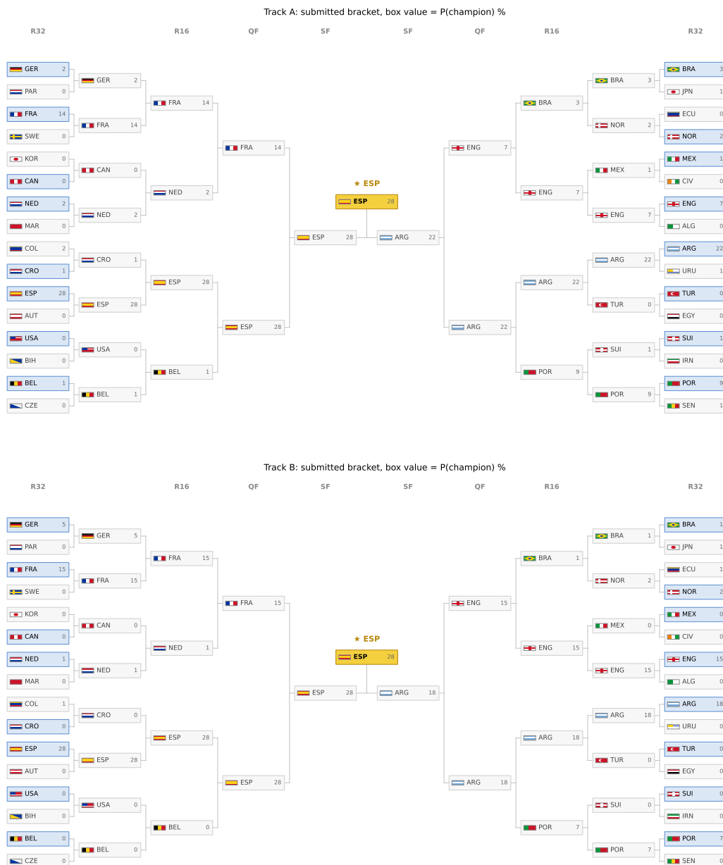
Figure 19: The submitted bracket re-valued by champion probability under Track A (top) and Track B (bottom) at live edition M047; the gold box is each track's most likely champion and greyed boxes are teams eliminated by confirmed results. The locked submitted bracket is Figure 18.
