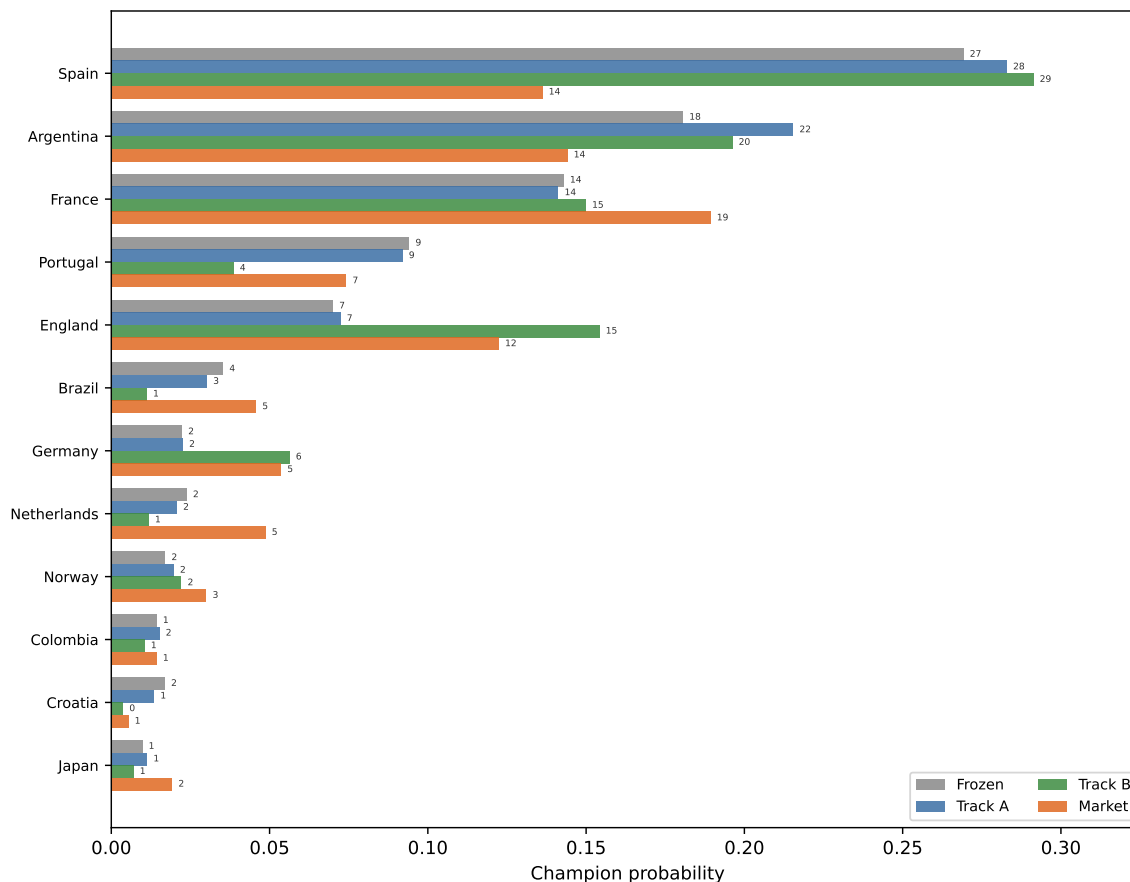
Figure 4: Champion probability, four ways: Frozen / Track A / Track B / Market, top twelve teams (live edition M047)
