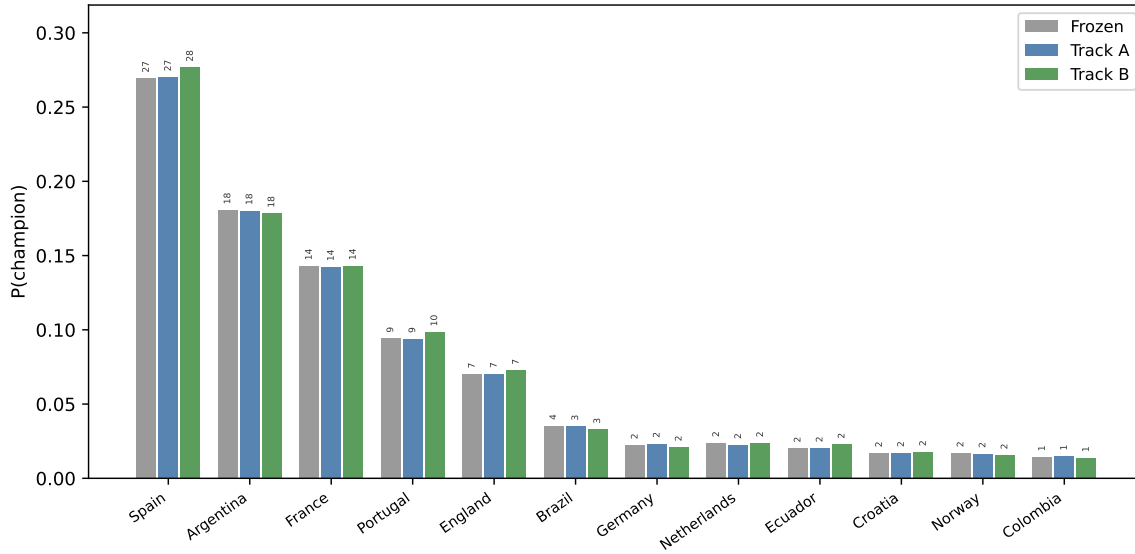
Figure 2: Champion probability distribution, conditioned on 4 results (live edition M004)
