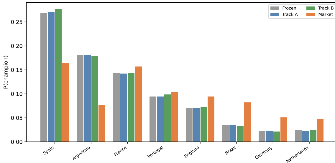
Figure 7: Four-bar champion probability: Frozen / Track A / Track B / Market, top contenders (live edition M004)
