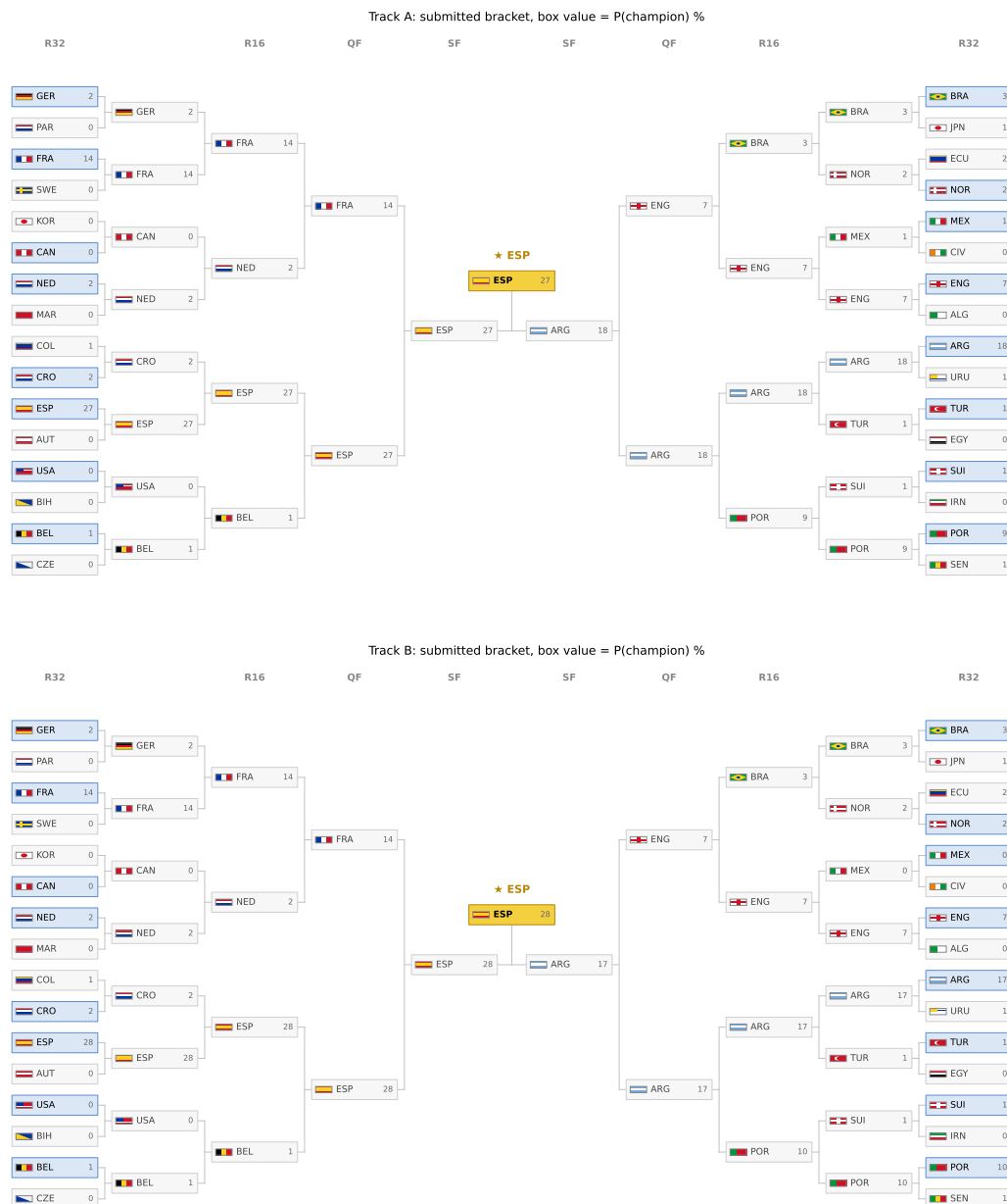
Figure 23: The submitted bracket re-valued by champion probability under Track A (top) and Track B (bottom) at live edition M004; the gold box is each track's most likely champion and greyed boxes are teams eliminated by confirmed results. The locked submitted bracket is Figure 22.
