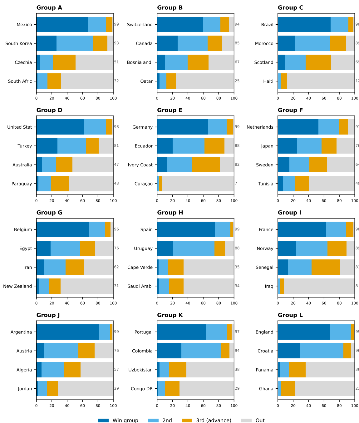
Figure 20: Qualification probability by team — Track A (conditioned on 4 results, June 10 ratings frozen; live edition M004)
