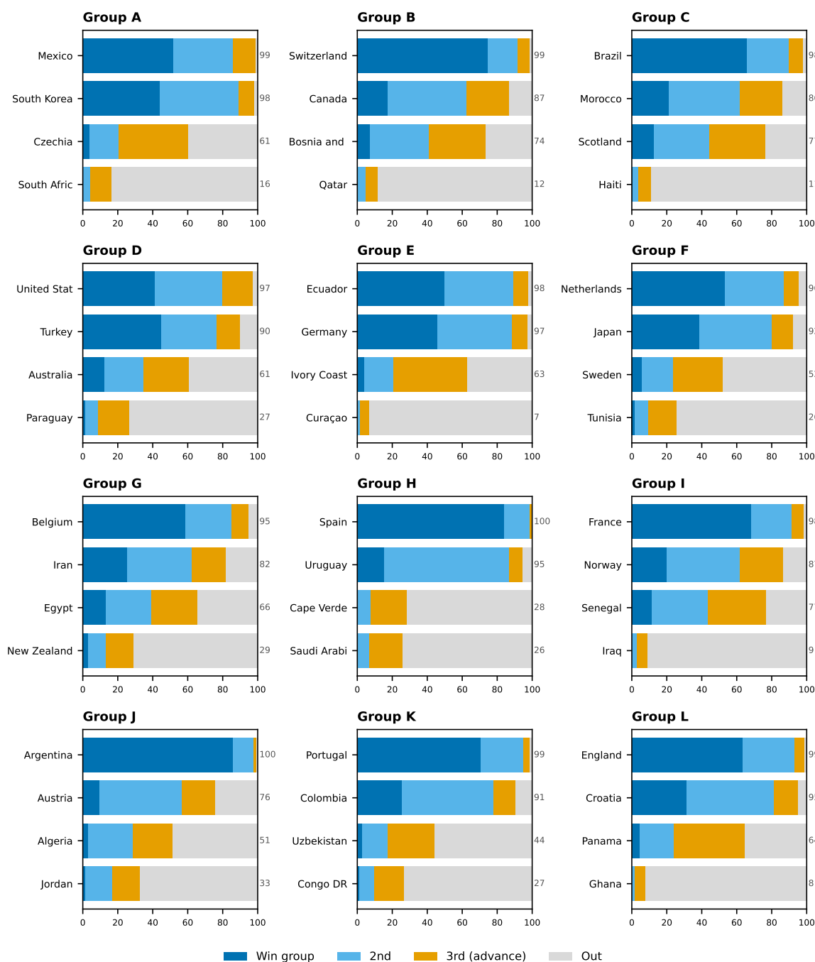
Figure 21: Qualification probability by team — Track B (result-conditioning + live Elo + bookmaker odds; live edition M004)
