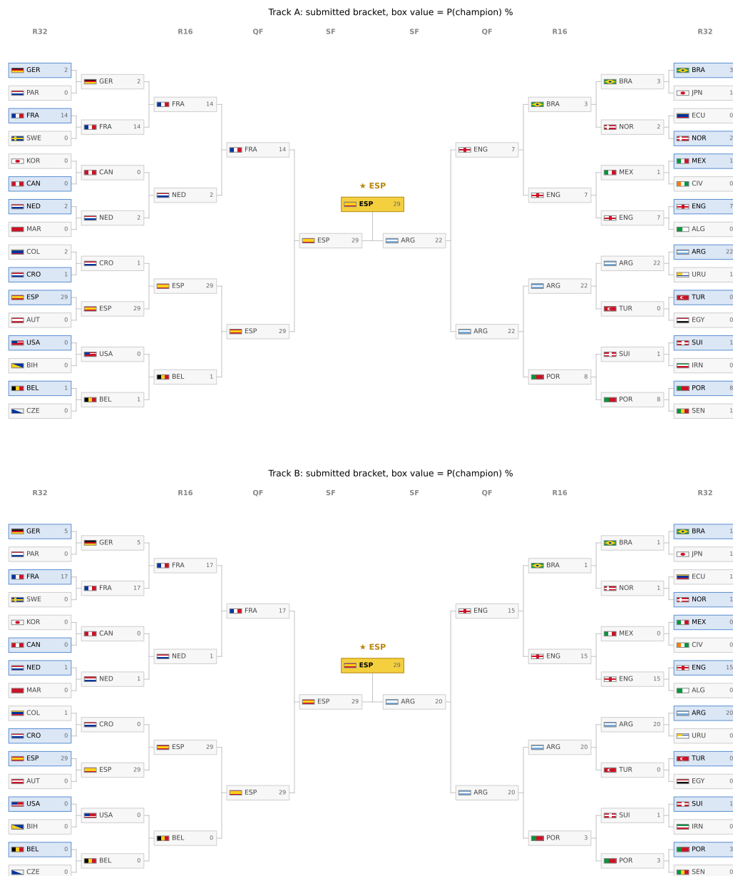
Figure 19: The submitted bracket re-valued by champion probability under Track A (top) and Track B (bottom) at live edition M043; the gold box is each track's most likely champion and greyed boxes are teams eliminated by confirmed results. The locked submitted bracket is Figure 18.
