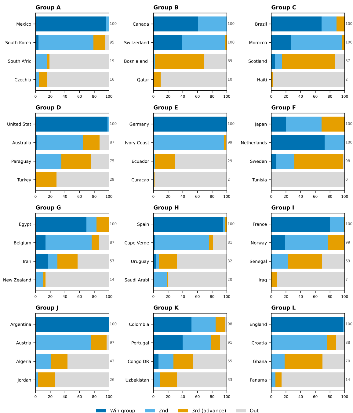
Figure 17: Qualification probability by team — Track B (result-conditioning + live Elo + bookmaker odds; live edition M043)
