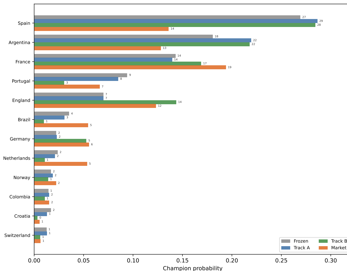
Figure 4: Champion probability, four ways: Frozen / Track A / Track B / Market, top twelve teams (live edition M043)
