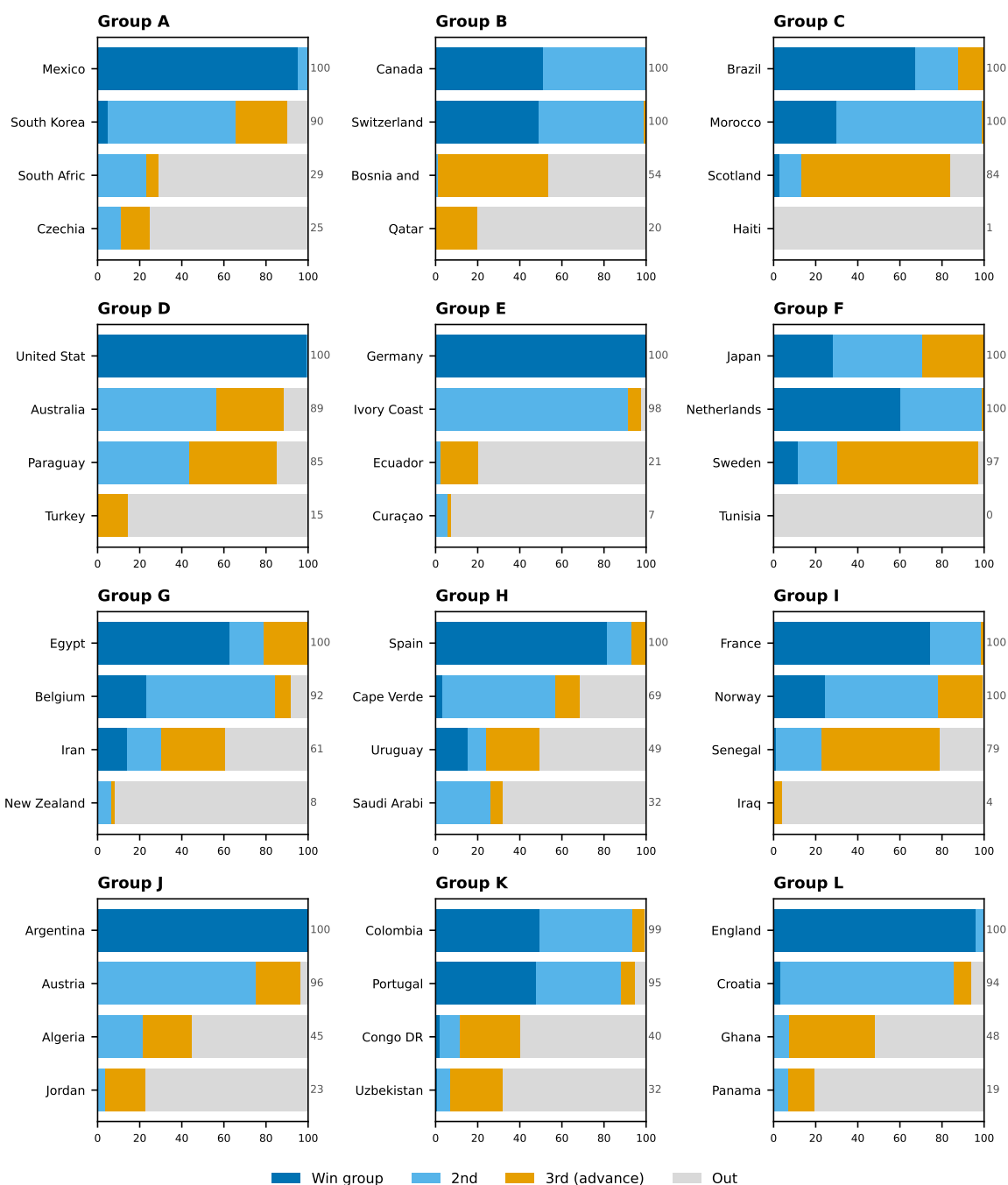
Figure 16: Qualification probability by team — Track A (conditioned on 41 results, June 10 ratings frozen; live edition M043)
