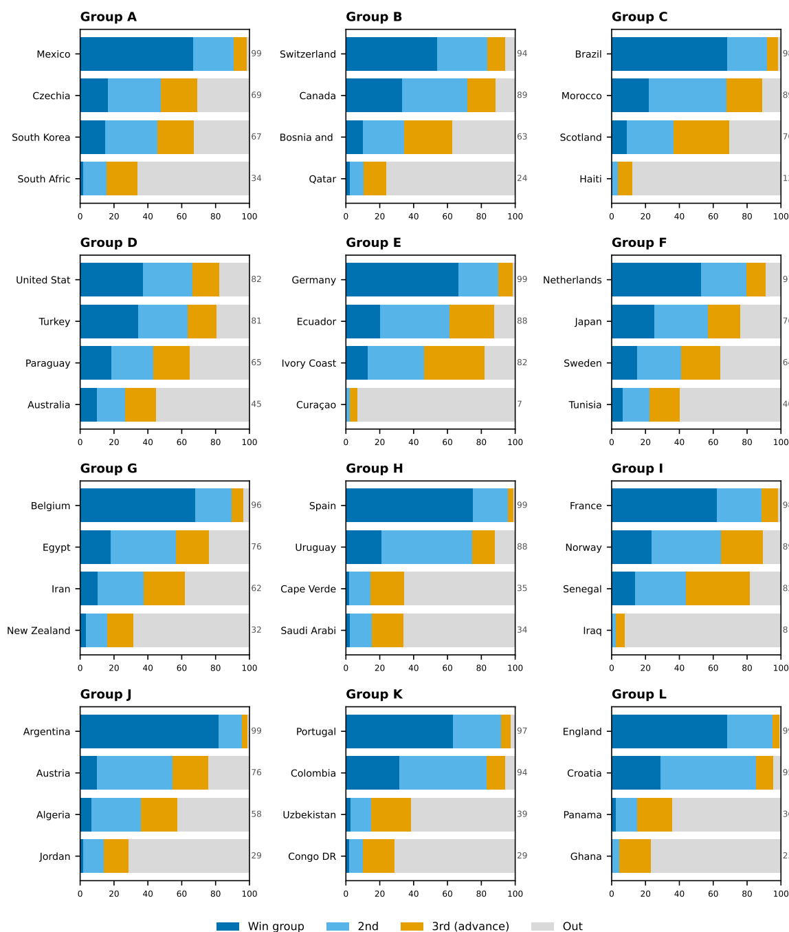
Figure 16: Qualification probability by team — Track A (conditioned on 1 results, June 10 ratings frozen; live edition M001)
