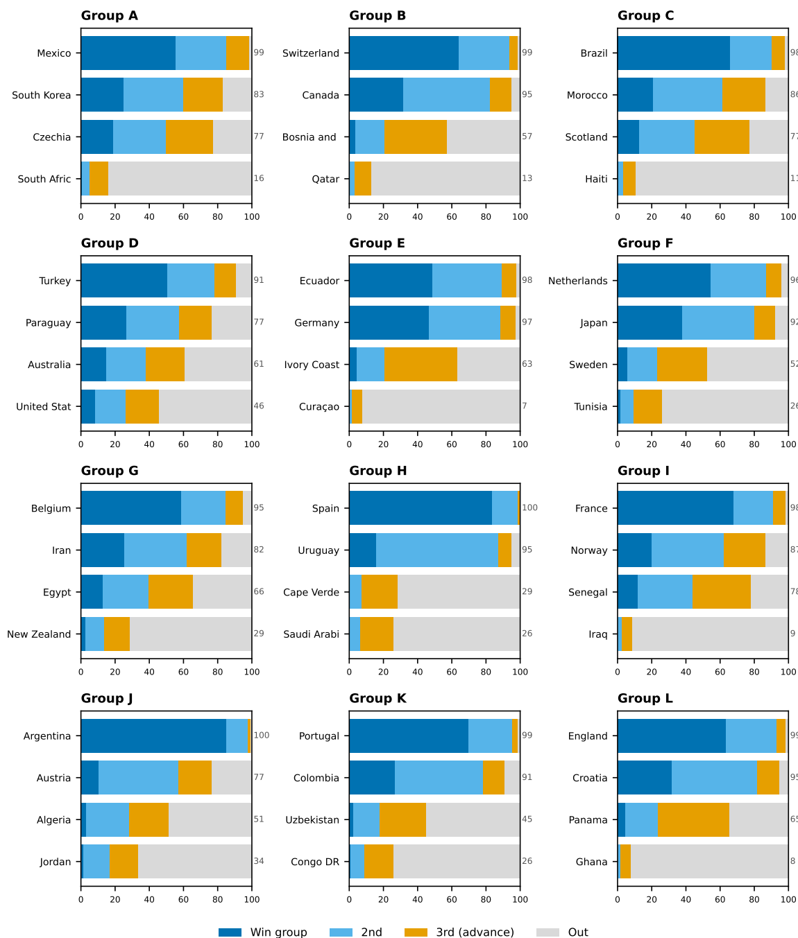
Figure 17: Qualification probability by team — Track B (result-conditioning + live Elo + bookmaker odds; live edition M001)
