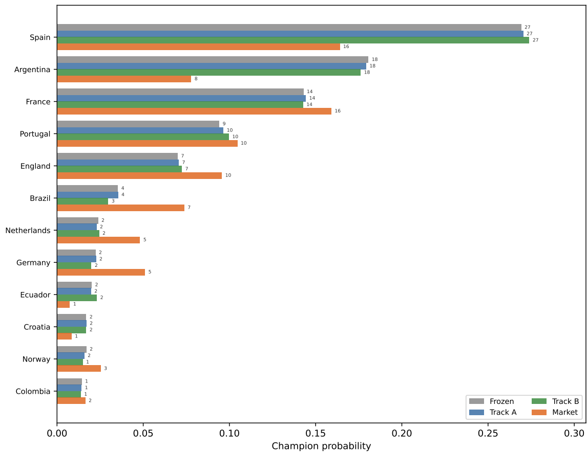
Figure 4: Champion probability, four ways: Frozen / Track A / Track B / Market, top twelve teams (live edition M008)
