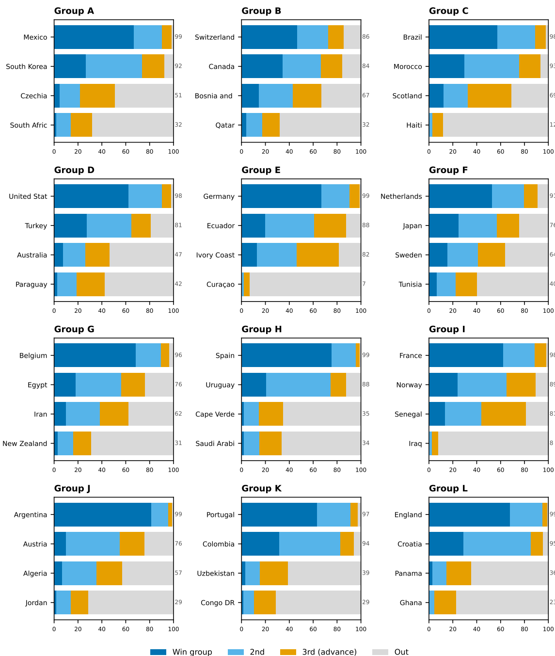
Figure 16: Qualification probability by team — Track A (conditioned on 6 results, June 10 ratings frozen; live edition M008)
