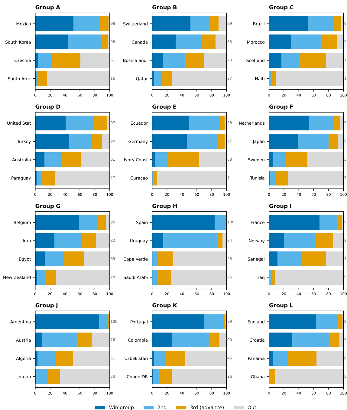
Figure 17: Qualification probability by team — Track B (result-conditioning + live Elo + bookmaker odds; live edition M008)
