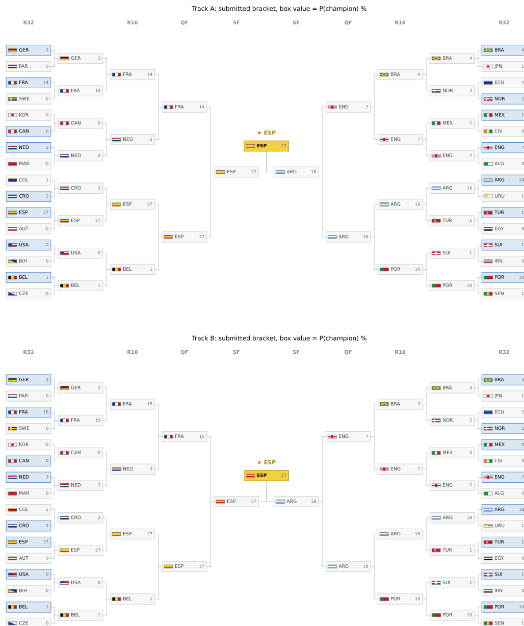
Figure 19: The submitted bracket re-valued by champion probability under Track A (top) and Track B (bottom) at live edition M008; the gold box is each track’s most likely champion and greyed boxes are teams eliminated by confirmed results. The locked submitted bracket is Figure 18.
