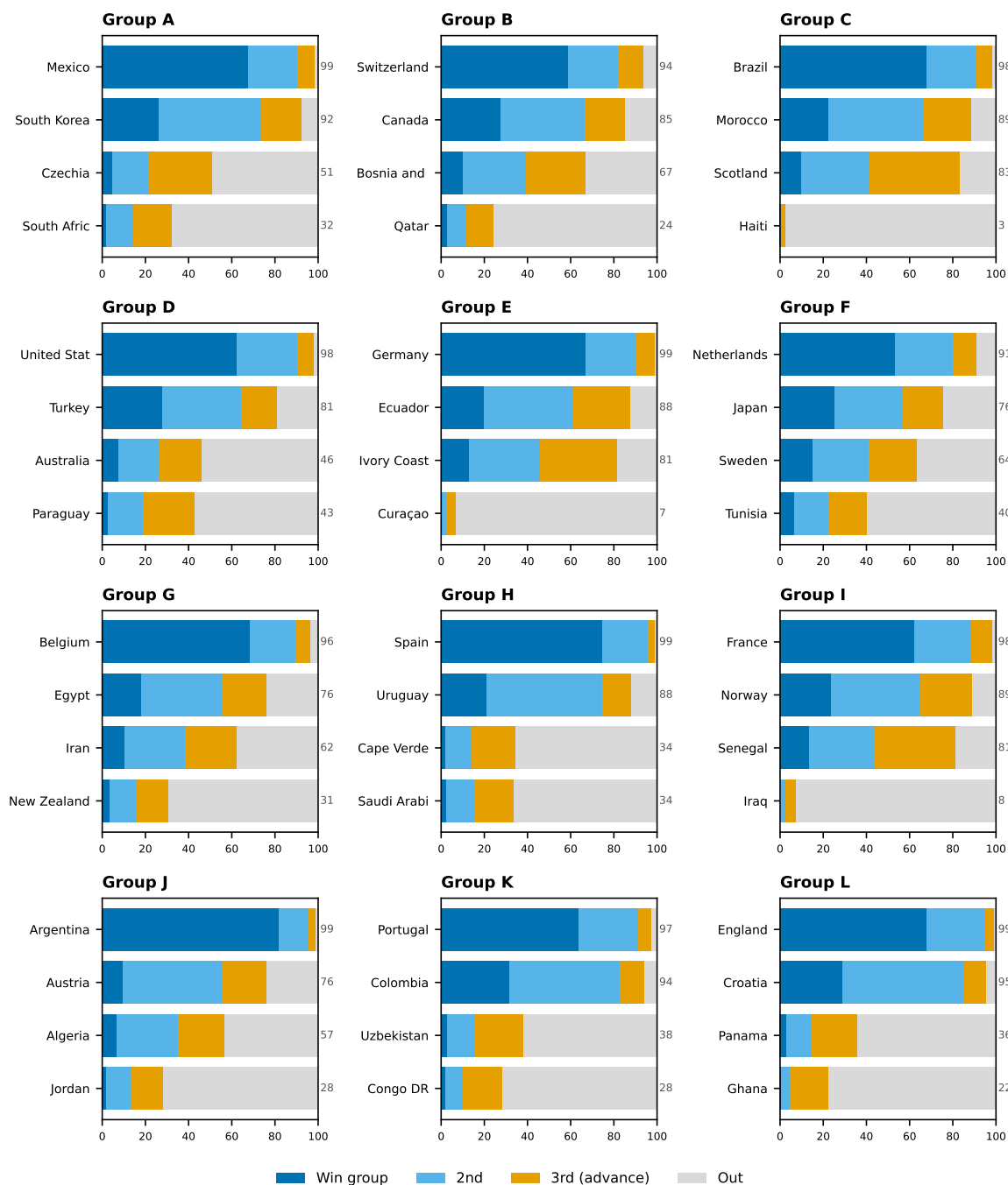
Figure 16: Qualification probability by team — Track A (conditioned on 5 results, June 10 ratings frozen; live edition M005)
