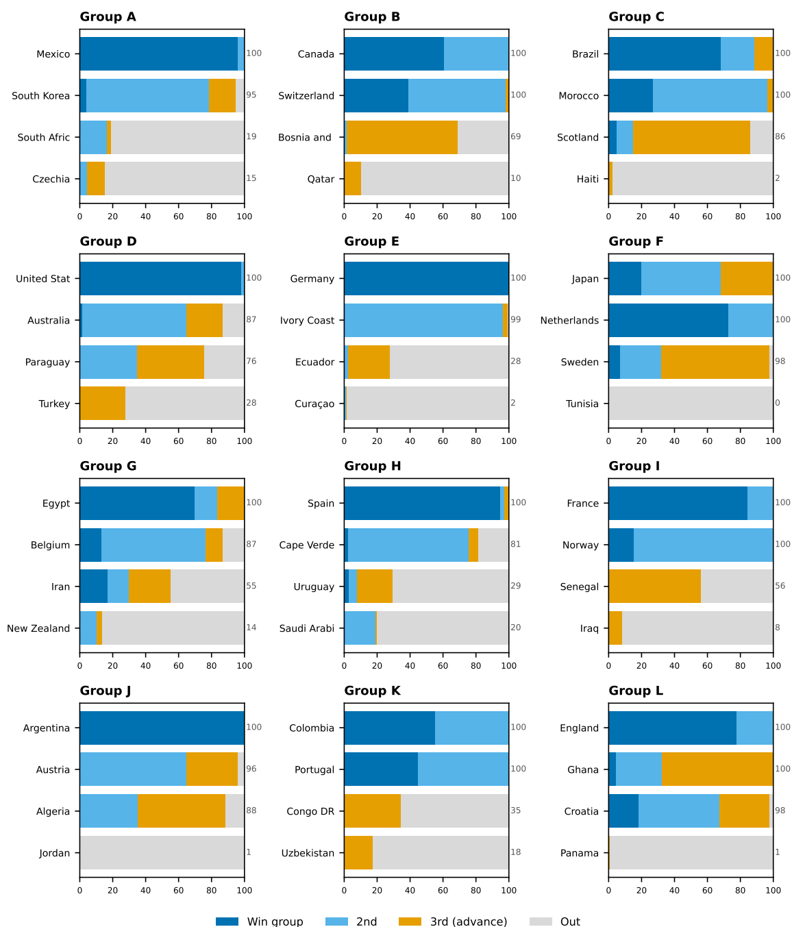
Figure 17: Qualification probability by team — Track B (result-conditioning + live Elo + bookmaker odds; live edition M048)
