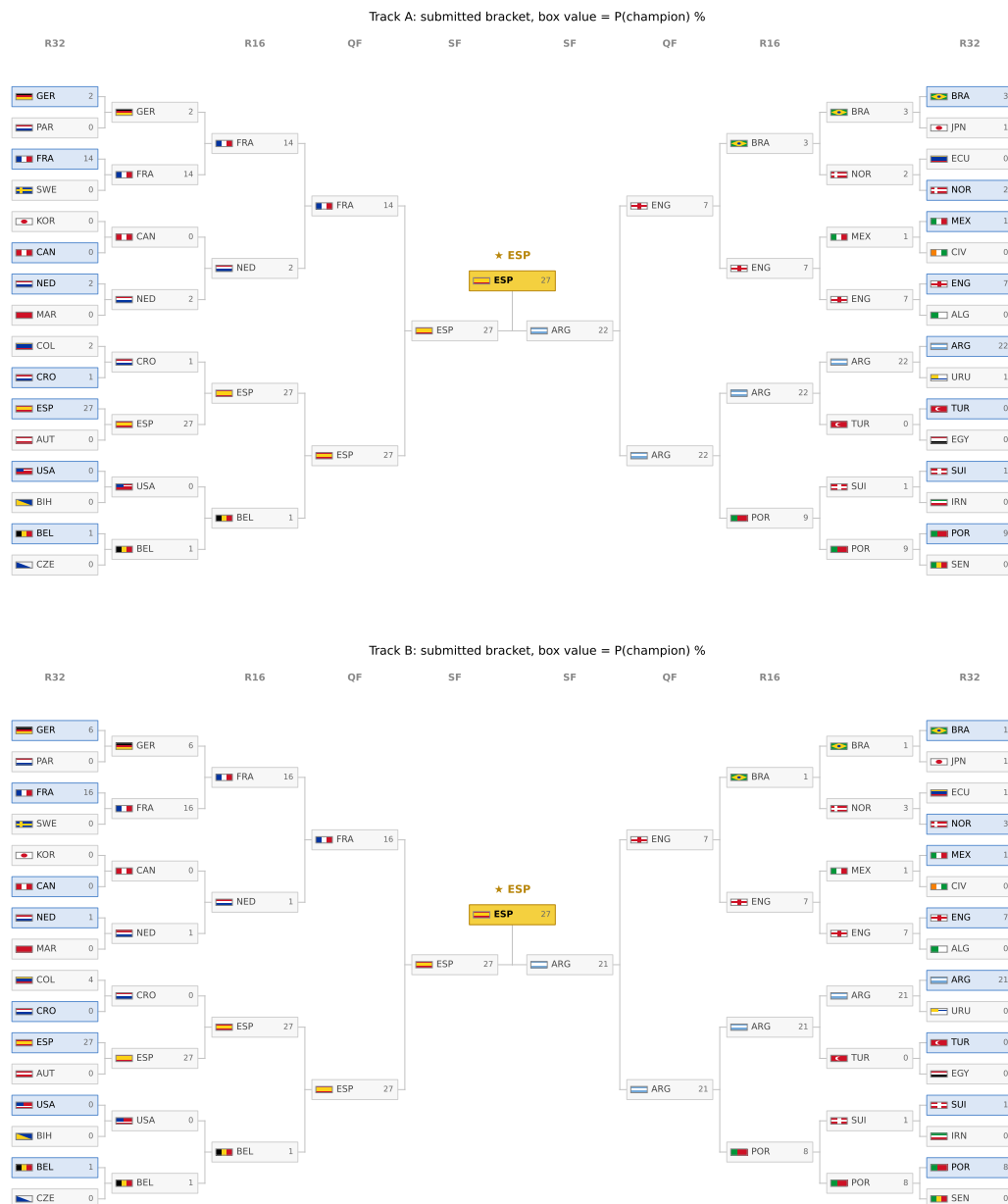
Figure 19: The submitted bracket re-valued by champion probability under Track A (top) and Track B (bottom) at live edition M048; the gold box is each track's most likely champion and greyed boxes are teams eliminated by confirmed results. The locked submitted bracket is Figure 18.
