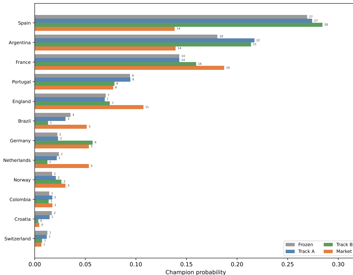
Figure 4: Champion probability, four ways: Frozen / Track A / Track B / Market, top twelve teams (live edition M048)
