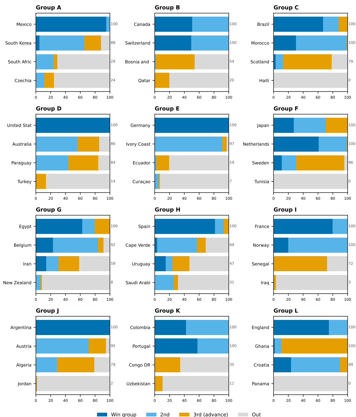
Figure 16: Qualification probability by team — Track A (conditioned on 48 results, June 10 ratings frozen; live edition M048)
