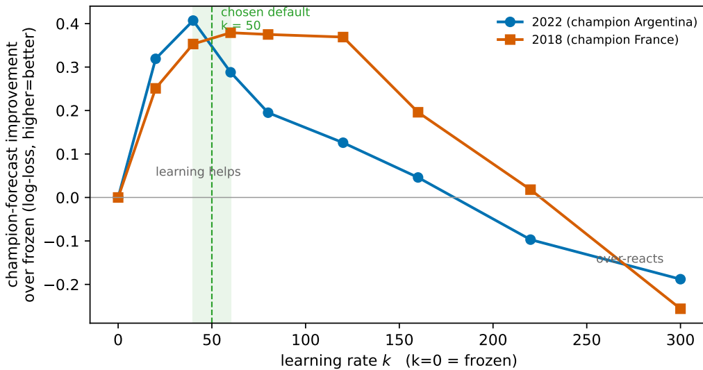
Figure 21: Learning-rate sweep on two World Cups
