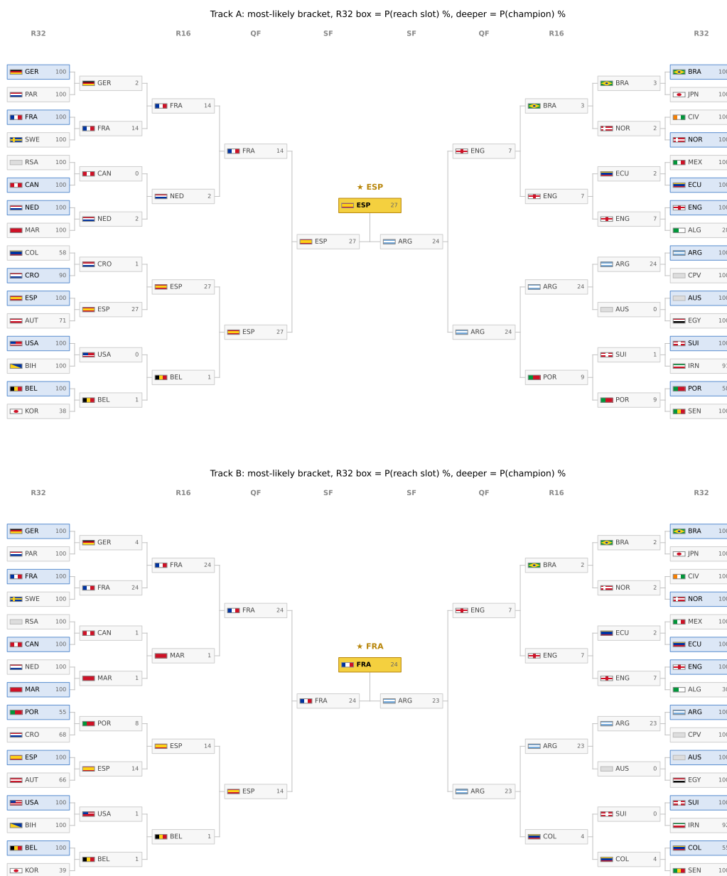
Figure 20: The most-likely bracket: the same submitted layout, but each Round-of-32 slot is re-filled with the team most likely to occupy it (rather than the locked pick) under Track A (top) and Track B (bottom) at live edition M067. Round-of-32 boxes show the probability that team reaches the slot; rounds past the Round of 32 trace the Elo most-likely path with boxes showing champion probability, and upgrade to exact per-slot occupancy once the knockout draw is realised. Read against Figure 19, it shows where the live forecast would re-cast the bracket the entry locked in.
