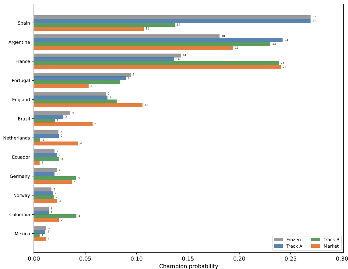
Figure 4: Champion probability, four ways: Frozen / Track A / Track B / Market, top twelve teams (live edition M067)
