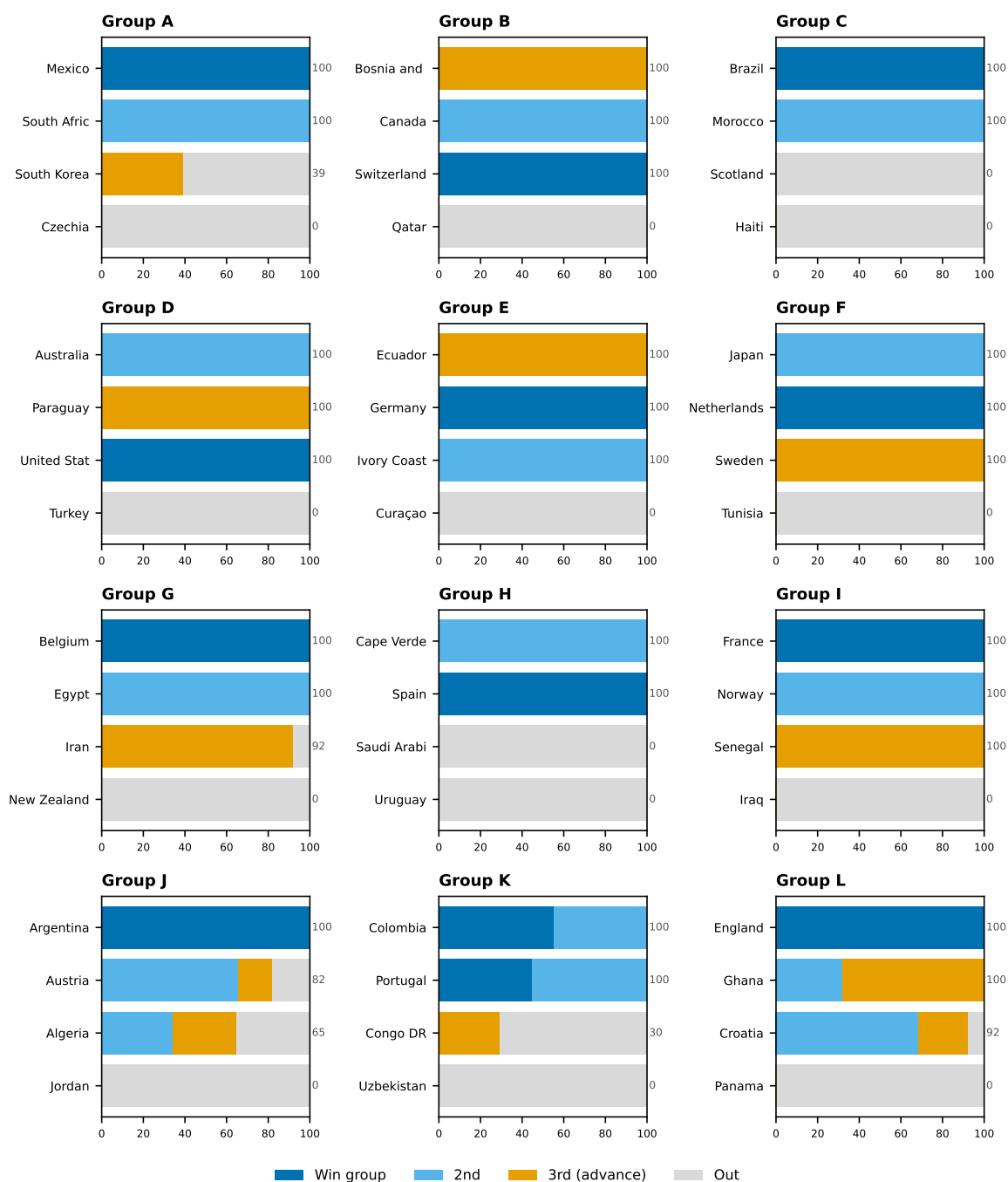
Figure 17: Qualification probability by team — Track B (result-conditioning + live Elo + bookmaker odds; live edition M067)
