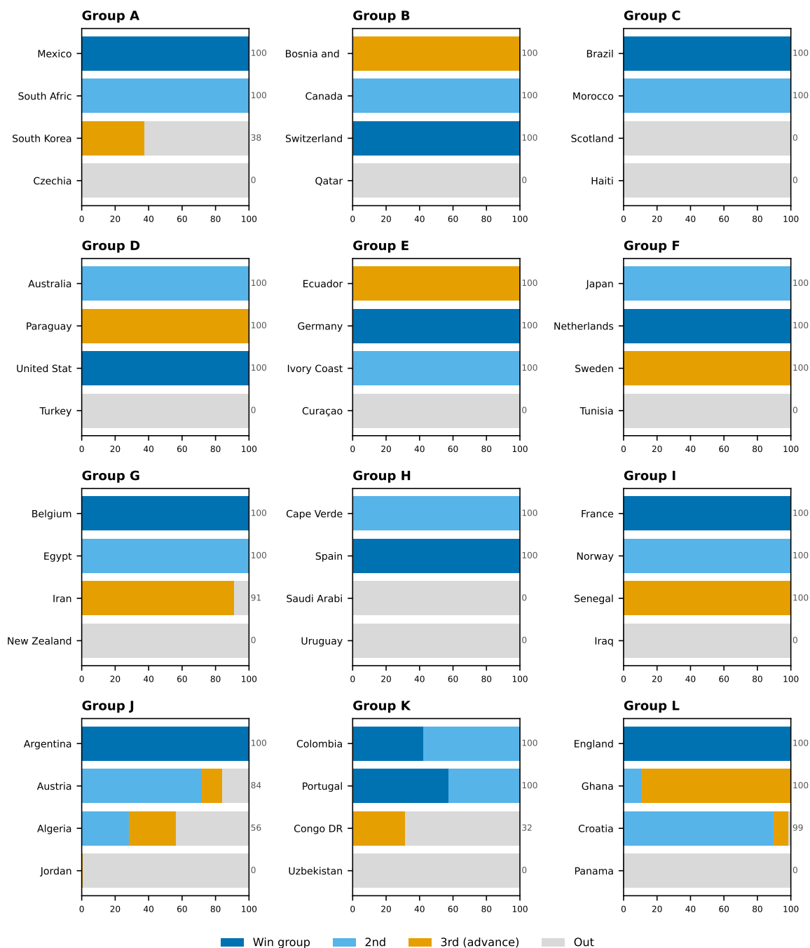
Figure 16: Qualification probability by team — Track A (conditioned on 67 results, June 10 ratings frozen; live edition M067)
