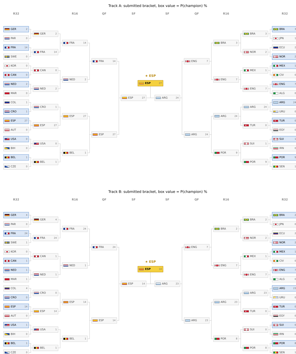
Figure 19: The submitted bracket re-valued by champion probability under Track A (top) and Track B (bottom) at live edition M067; the gold box is each track's most likely champion and greyed boxes are teams eliminated by confirmed results. The locked submitted bracket is Figure 18.
