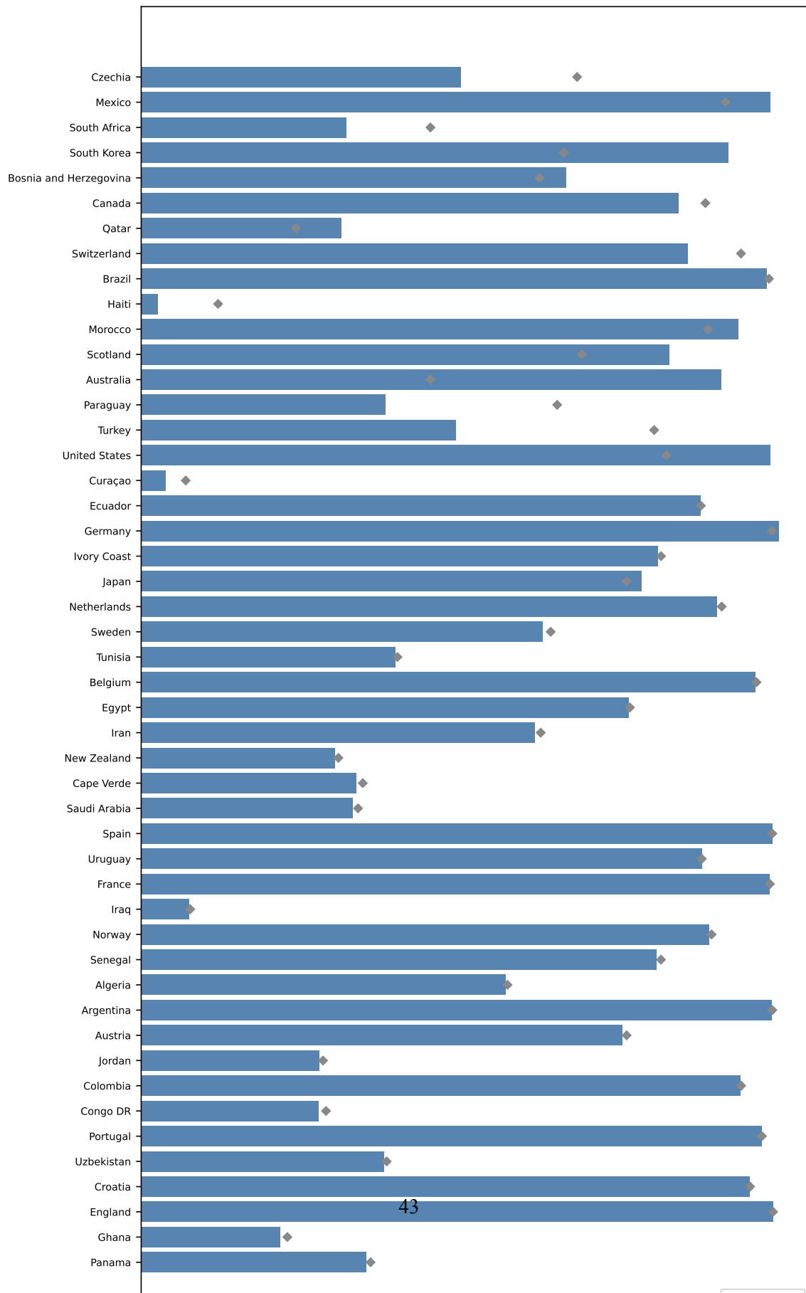
Figure 20: Qualification probability by team — Track A (conditioned on 10 results, June 10 ratings frozen; live edition M011)
