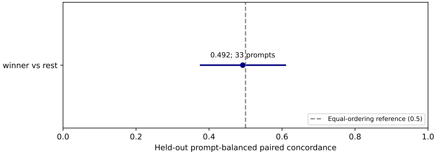
pickapic: frozen concept-score discrimination (95% intervals)
