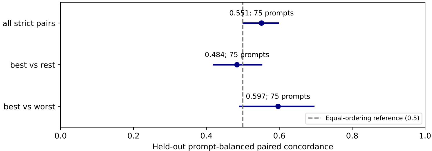
imagereward: frozen concept-score discrimination (95% intervals)
