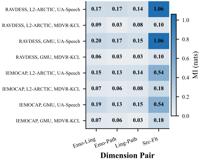
Dataset Combination
