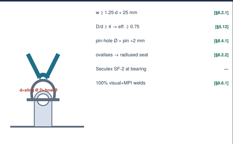
DETAIL B — HULL-EYE / SLING BEARING (§8.2)
