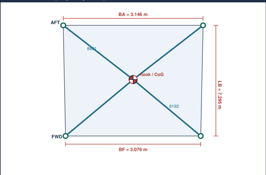
VIEW B — PLAN (lift-point pattern)
