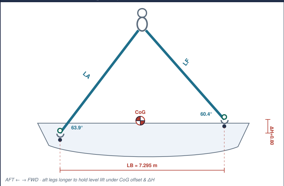
VIEW C — SIDE ELEVATION (profile)
