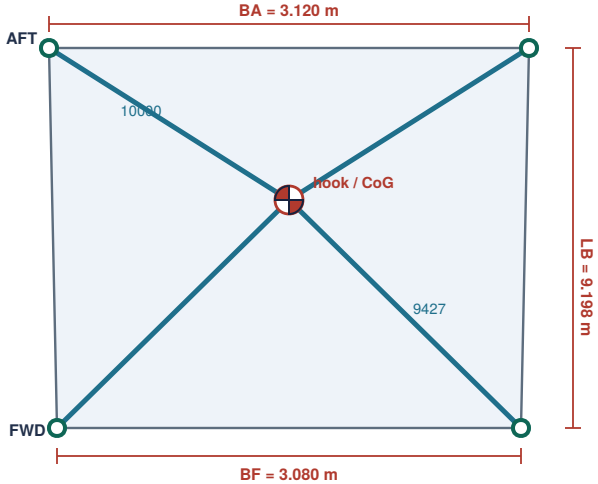
VIEW B — PLAN (lift-point pattern)
