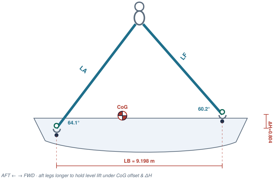
VIEW C — SIDE ELEVATION (profile)
