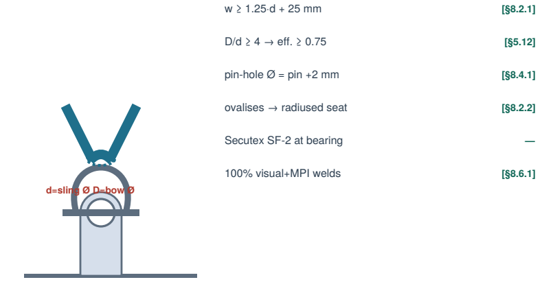
DETAIL B — HULL-EYE / SLING BEARING (§8.2)
