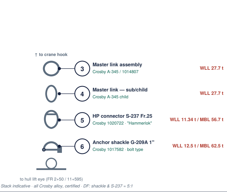
DETAIL B — HULL-EYE / SLING BEARING (§8.2)
