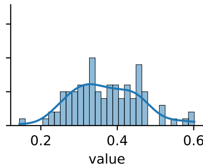
blur_stength
