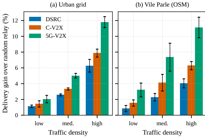
Fig. 4. End-to-end delivery gain of stability-aware relay selection over random selection in (a) the urban grid and (b) Vile Parle. Error bars show the 95% confidence interval over seeds.
