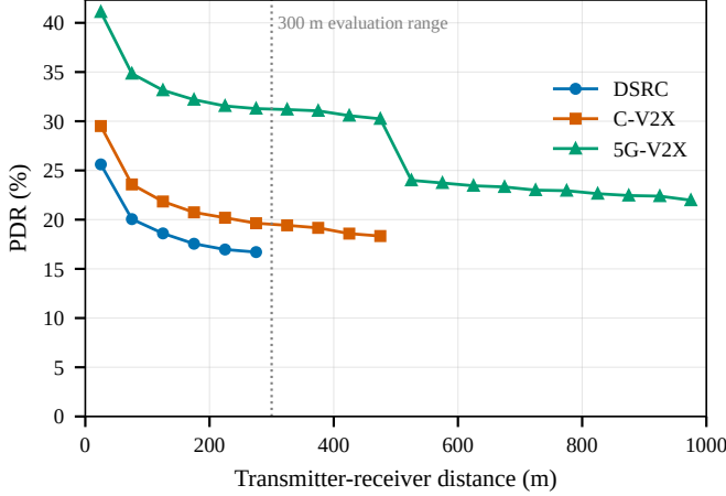
Fig. 2. PDR versus transmitter–receiver distance for DSRC, C-V2X, and 5G-V2X (Vile Parle, medium density, clear weather). The step of 5G-V2X at 500 m is caused by the reduced beamforming gain beyond that distance.
