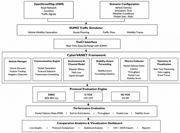
Fig. 1. Architecture of the CyberVANET framework. OpenStreetMap or synthetic networks feed SUMO, TraCI exposes vehicle state to the framework modules, and the protocol evaluation engine compares DSRC, C-V2X, and 5G-V2X under identical traffic.
