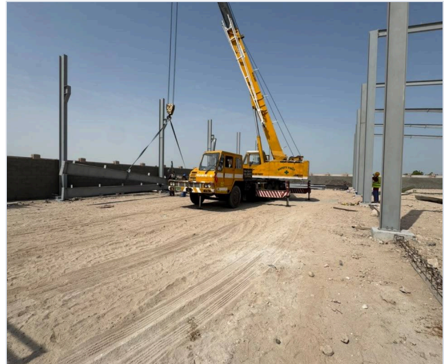
Column installation • anchoring
