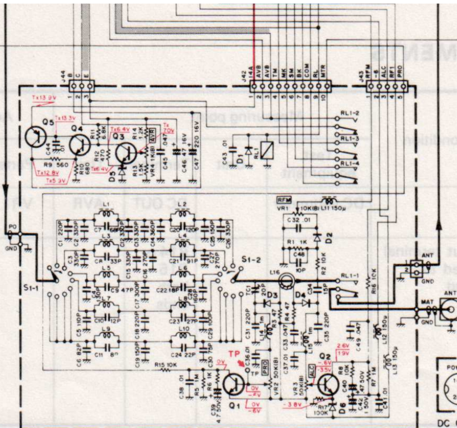
FILTER UNIT (X51-1170-00)
