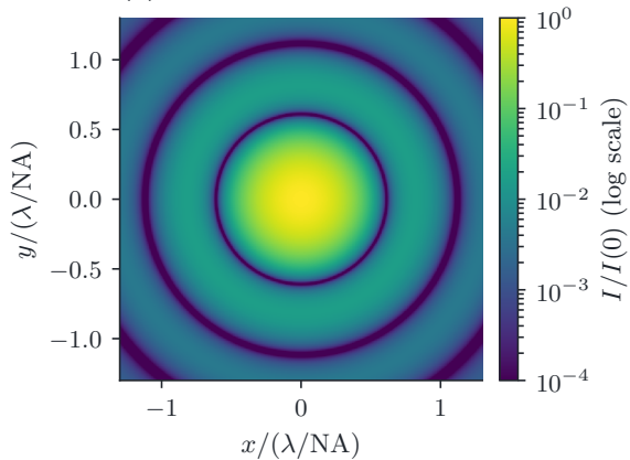
(a) Circular-pupil PSF
