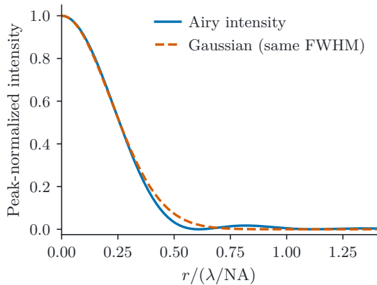
(b) Central-lobe approximation
