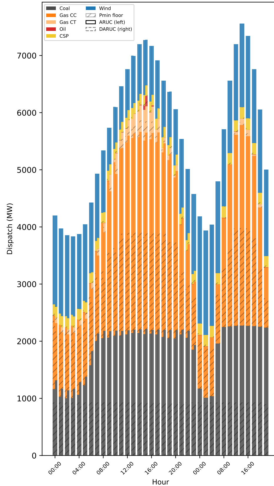
(b) Dispatch by fuel type
