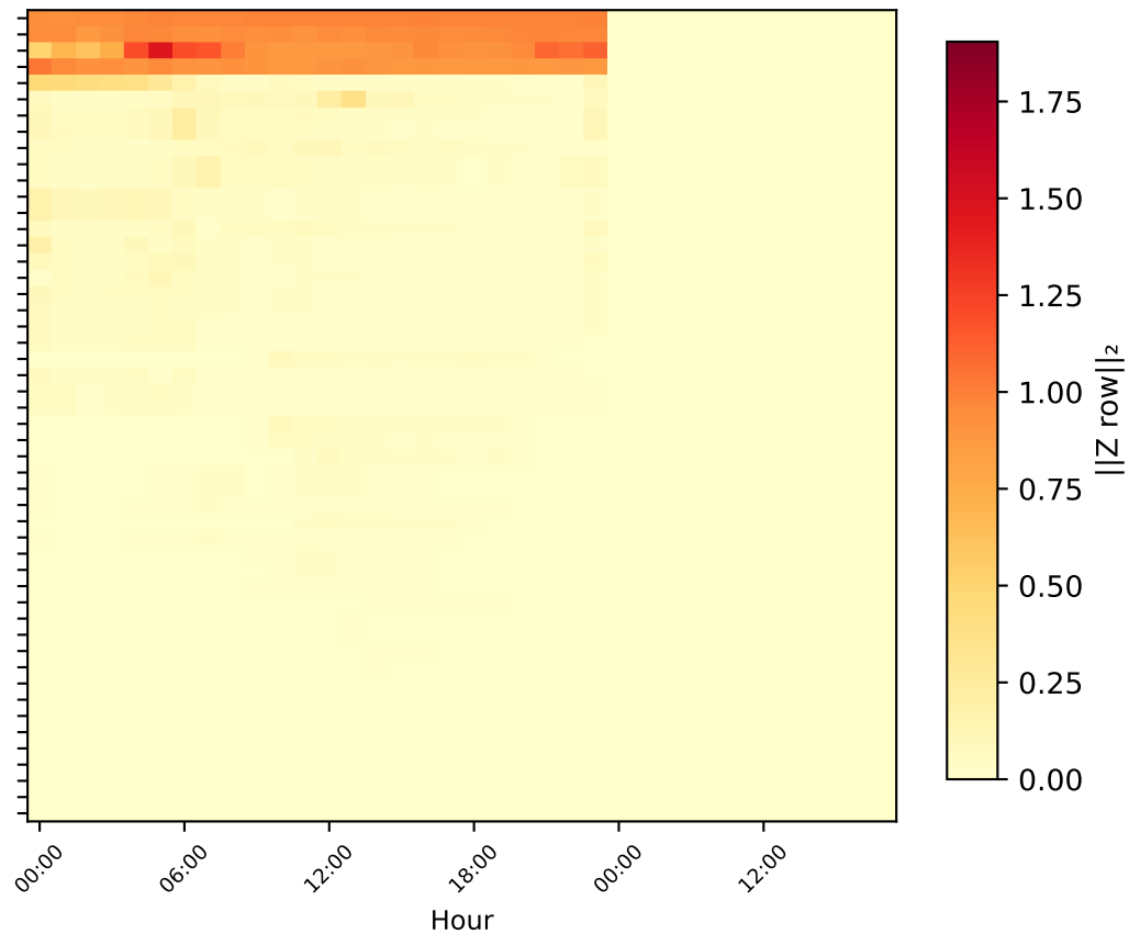
(b) DARUC: ||Z_{\text{row}}||
