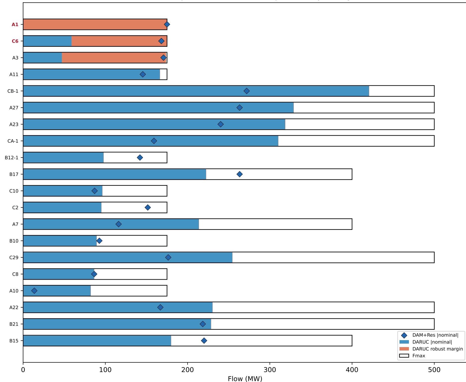
Flow Decomposition — Hour 17:00 (top 20 lines by loading)
