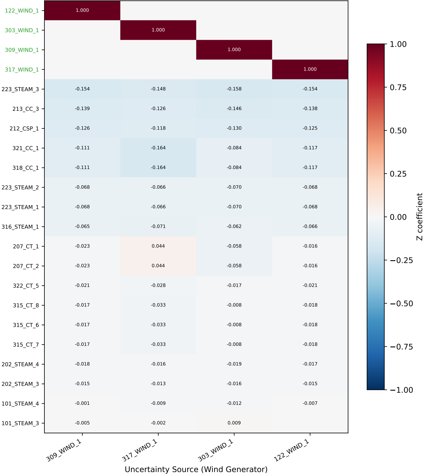
Option A: Z Matrix Heatmap — DARUC Hour 17 (22 gens with |Z| > 0.001 )
