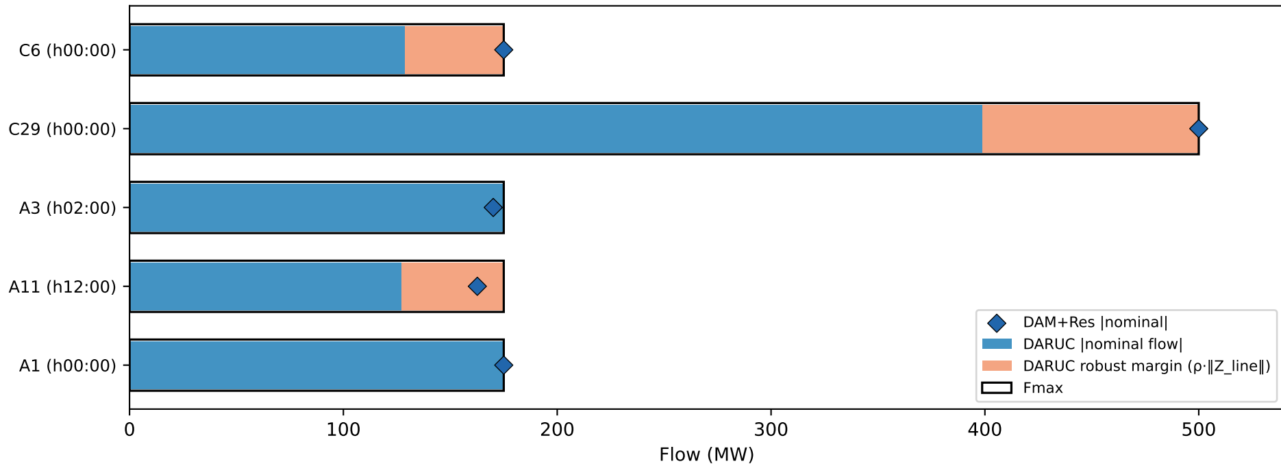
Flow Decomposition at Peak Hour (DARUC, Day 1)
