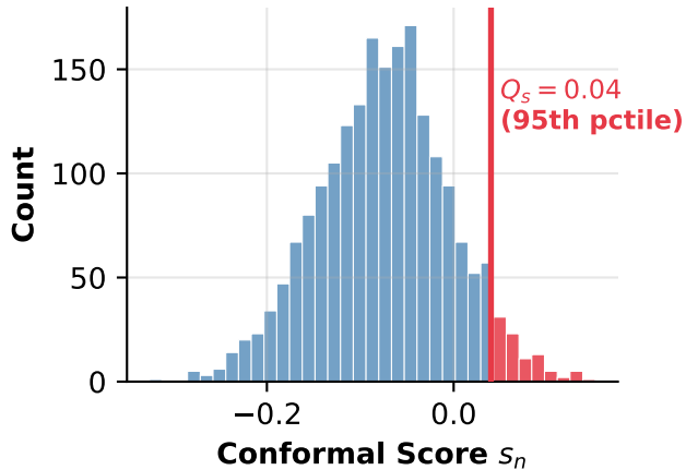
Calibration Scores
