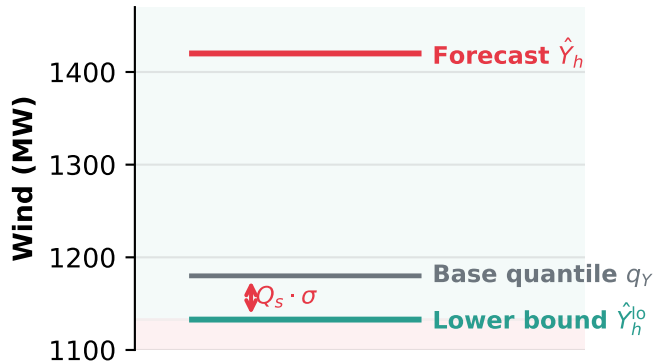
Conformal Correction
