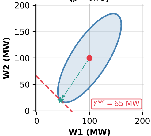
Positive correlation ( \rho = 0.75 )
