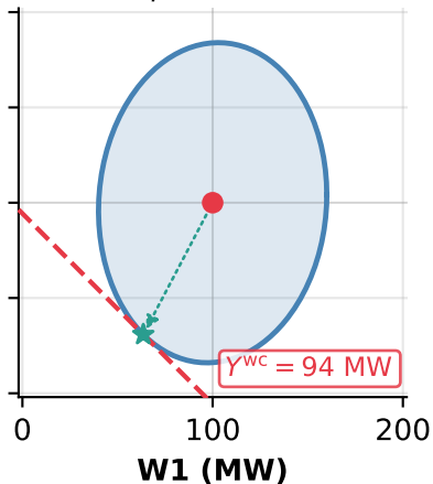
Weak correlation ( \rho = 0.05 )
