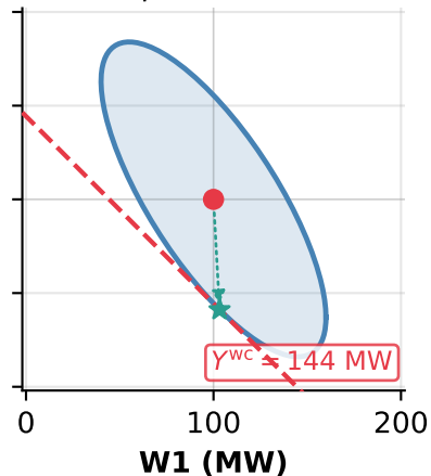
Negative correlation ( \rho = -0.75 )
