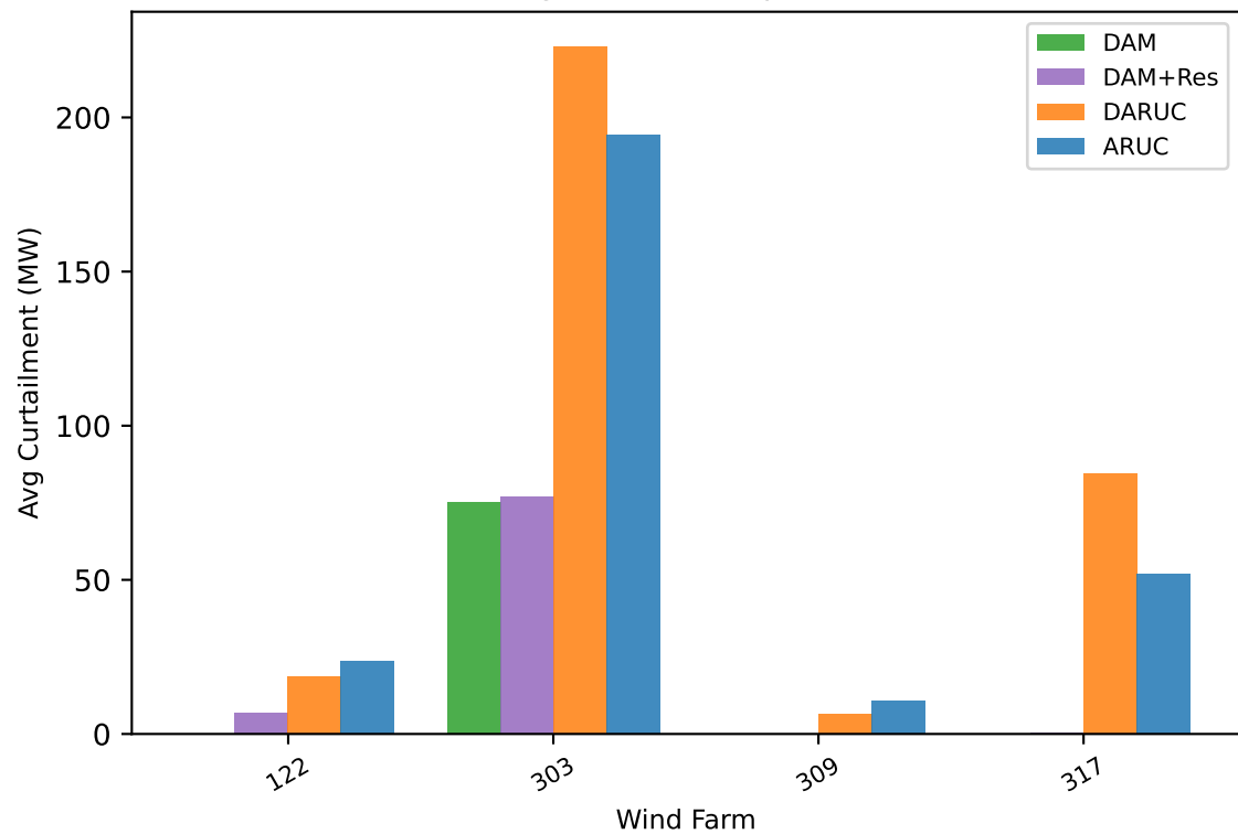
(b) Average curtailment per wind farm
