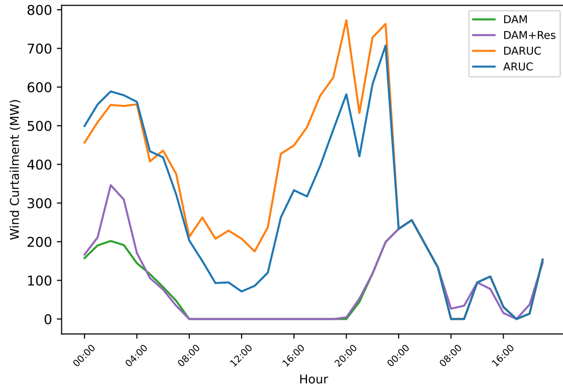
(a) Total wind curtailment over time
