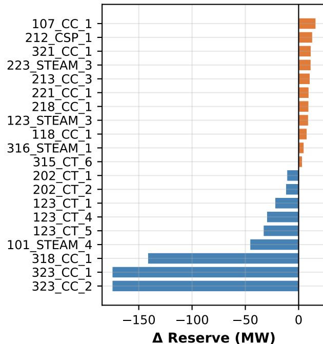
(c) DARUC-DAM at 16:00
