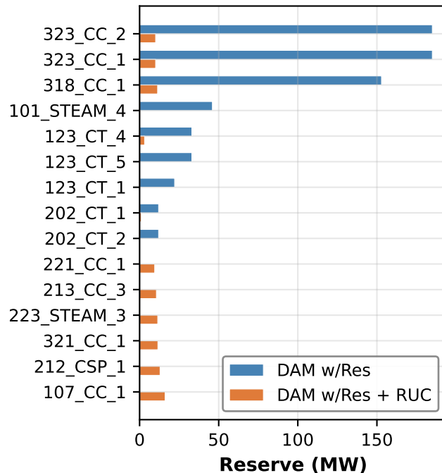
(b) Top units at 16:00
