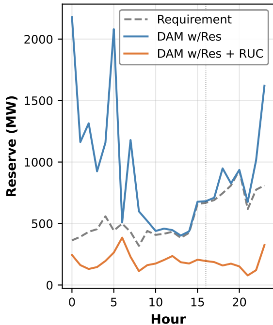
(a) System reserve by period
