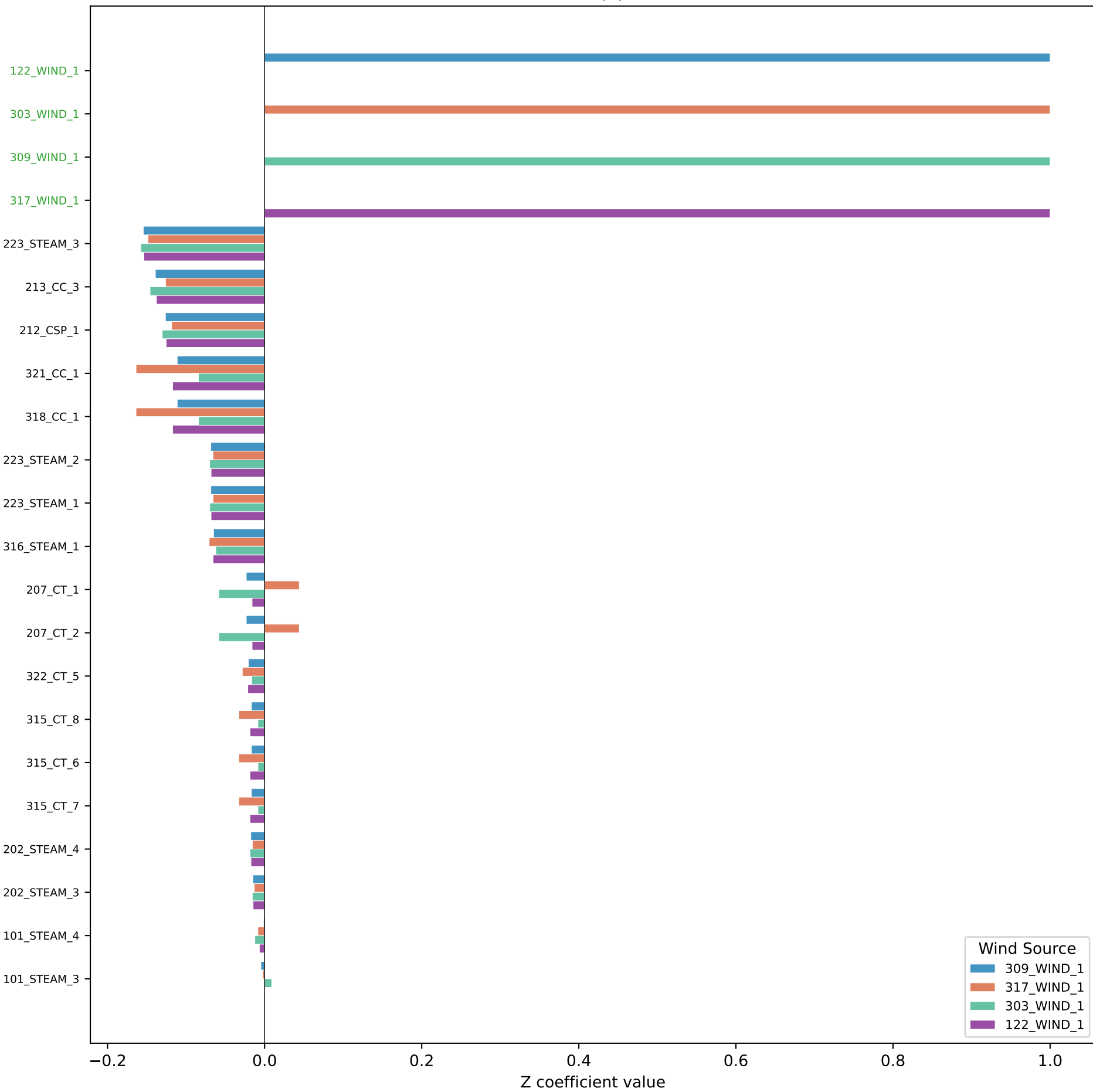
Option B: Z Coefficients by Wind Source — DARUC Hour 17 (22 gens with |Z| > 0.001 )
