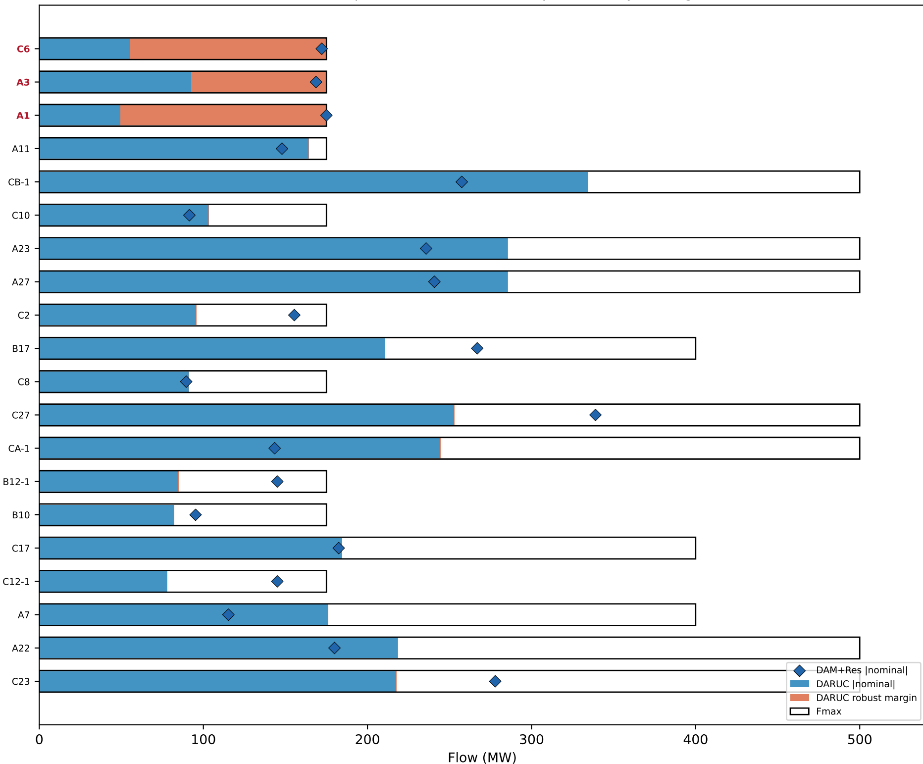
Flow Decomposition — Hour 16:00 (top 20 lines by loading)
