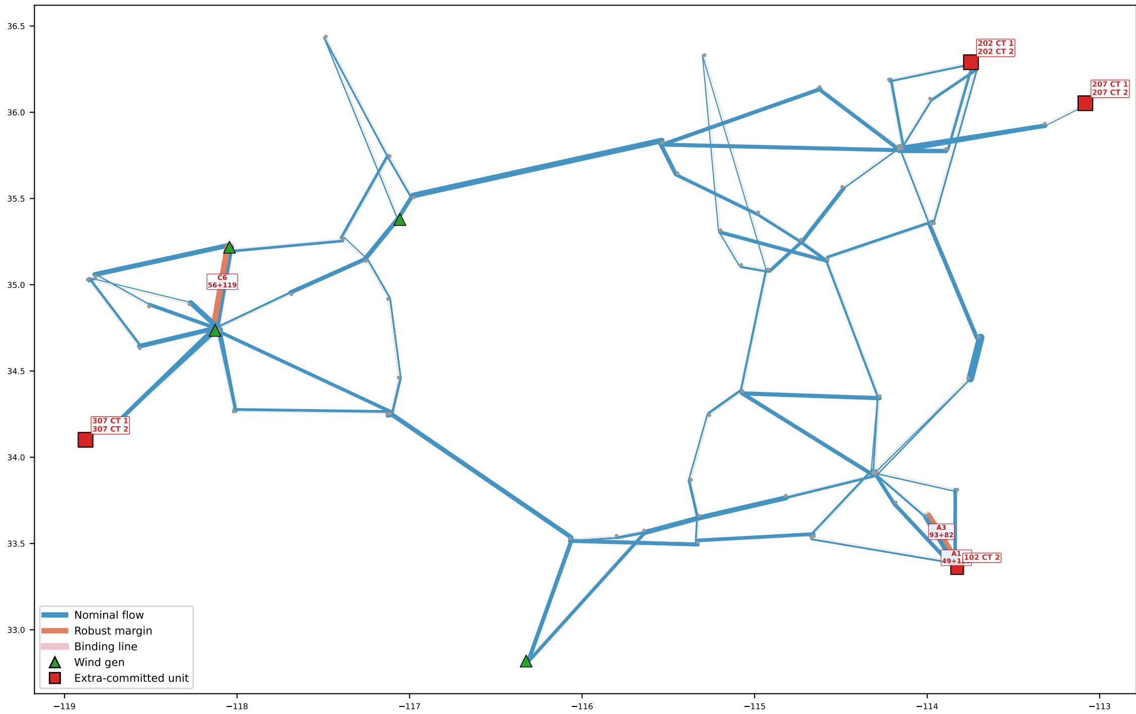
DARUC Flows + Extra Commitments — Hour 16:00
