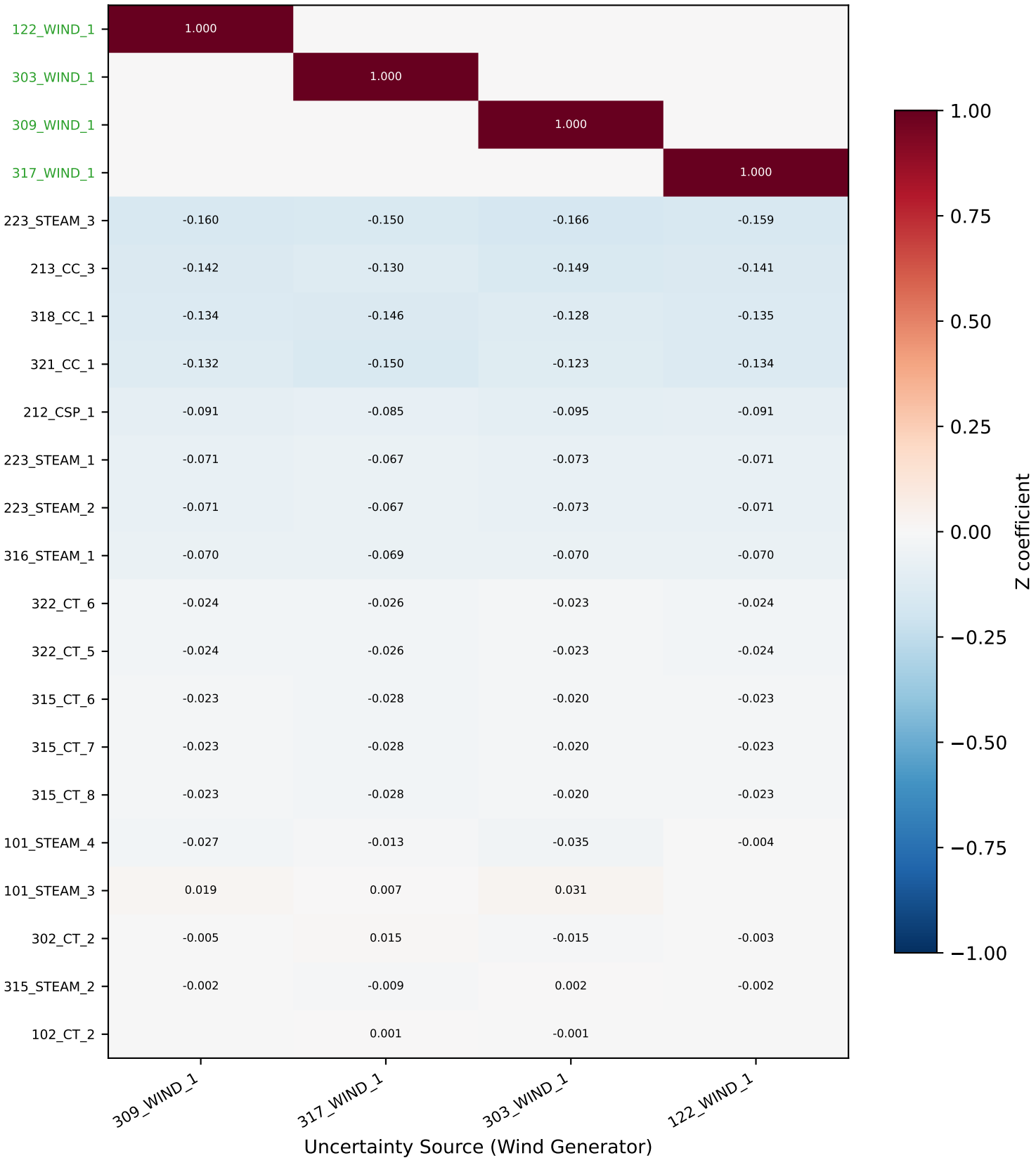
Option A: Z Matrix Heatmap — DARUC Hour 16 (22 gens with |Z| > 0.001 )
