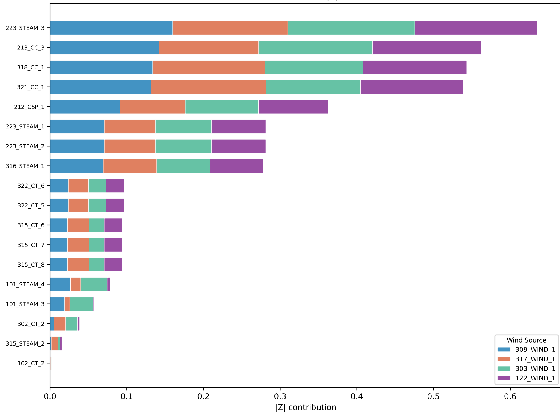
Thermal Response to Wind Uncertainty — DARUC Hour 16 (18 thermal gens with |Z| > 0.001 )
