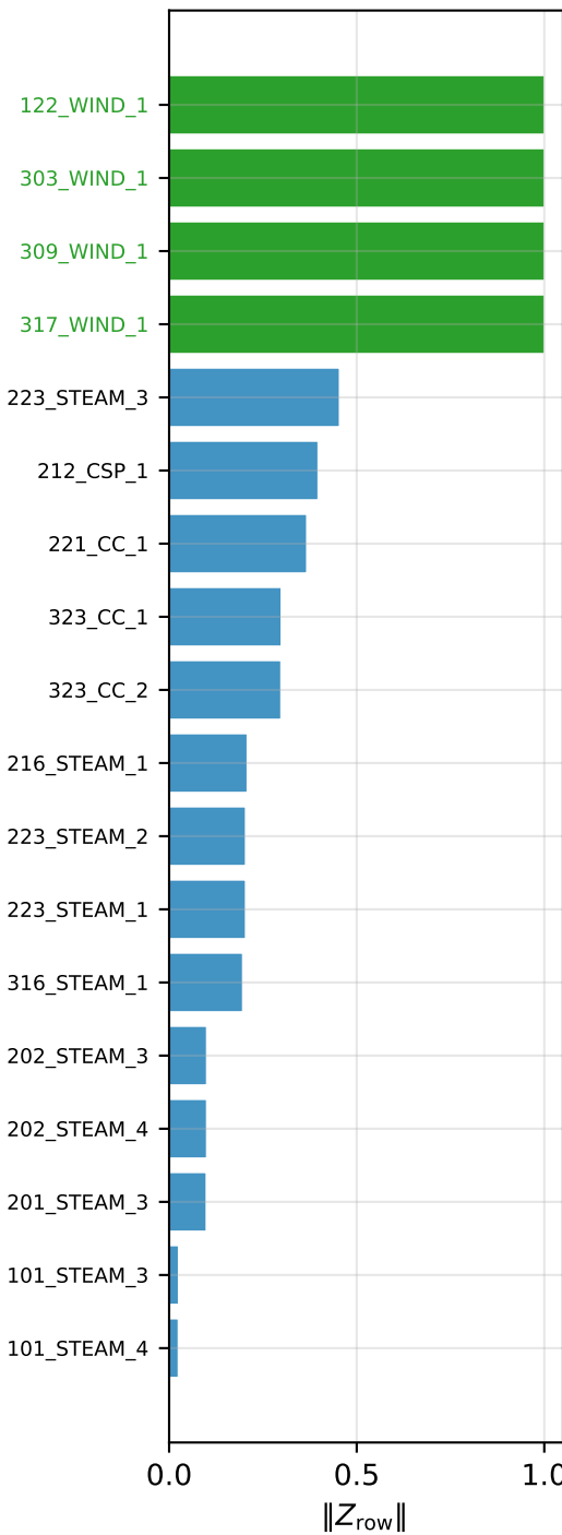
Row Norm
