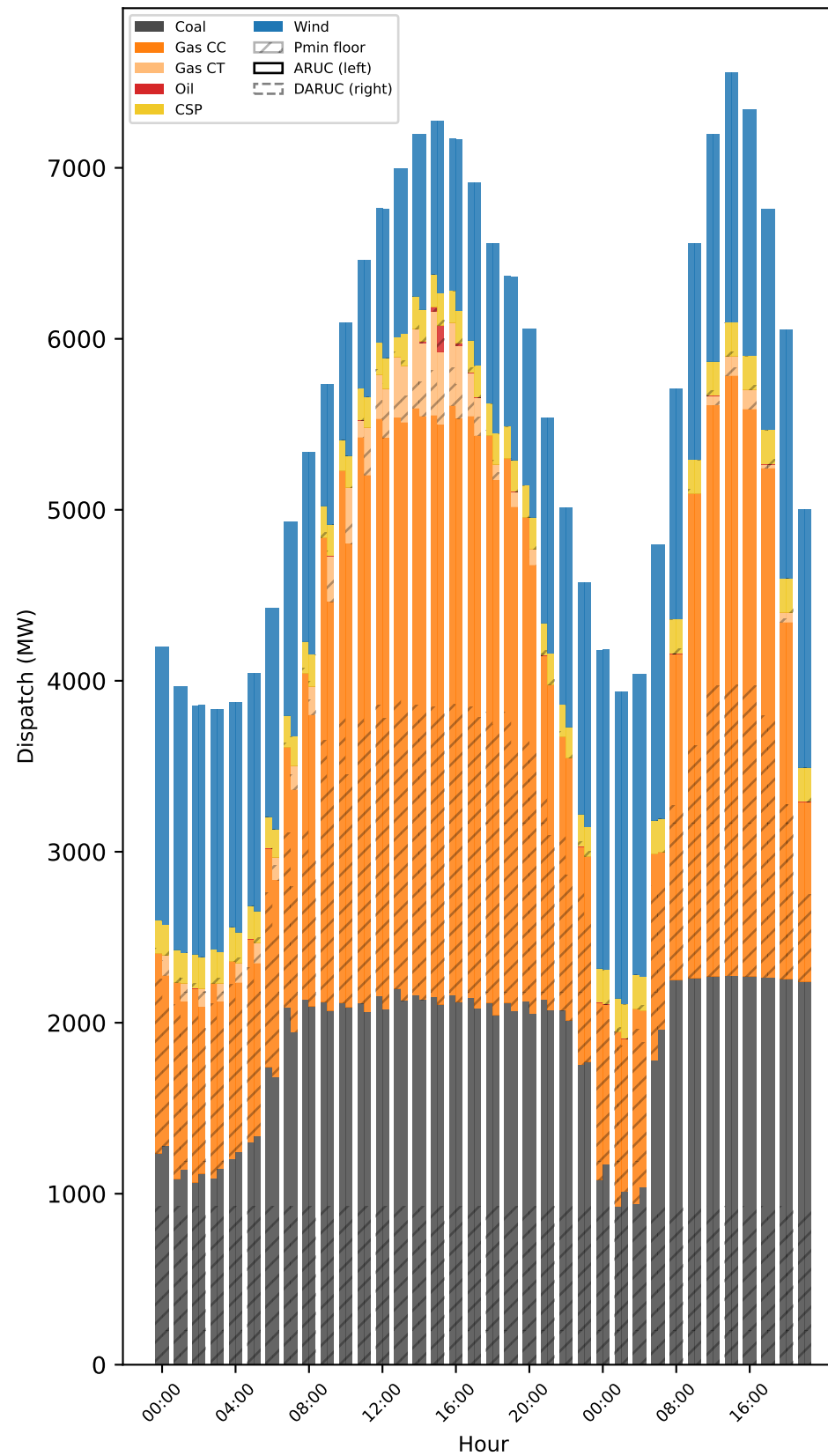
(b) Dispatch by fuel type
