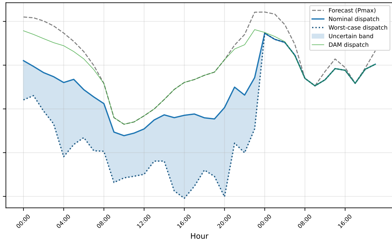
ARUC: Worst-Case Wind Dispatch
