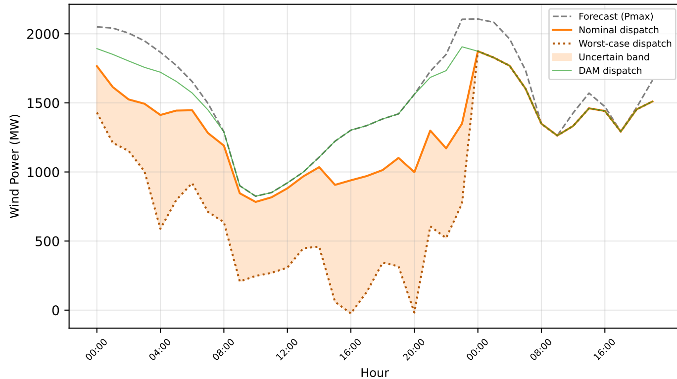
DARUC: Worst-Case Wind Dispatch
