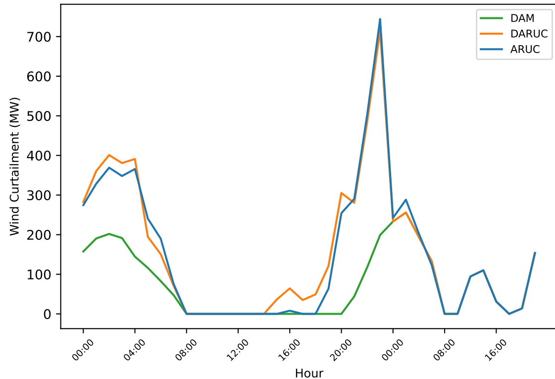
(a) Total wind curtailment over time
