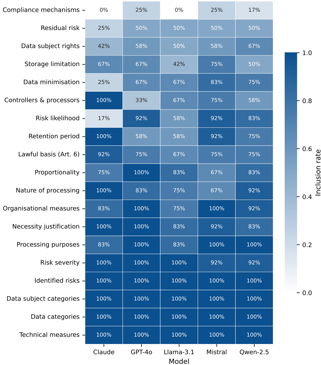
GDPR — Required field inclusion by model (mean across vagueness levels; sorted by lowest inclusion)
