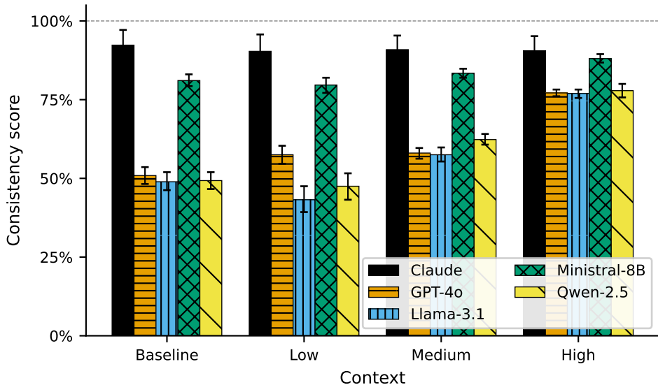
GDPR — Cross-run Consistency by Vagueness Level
