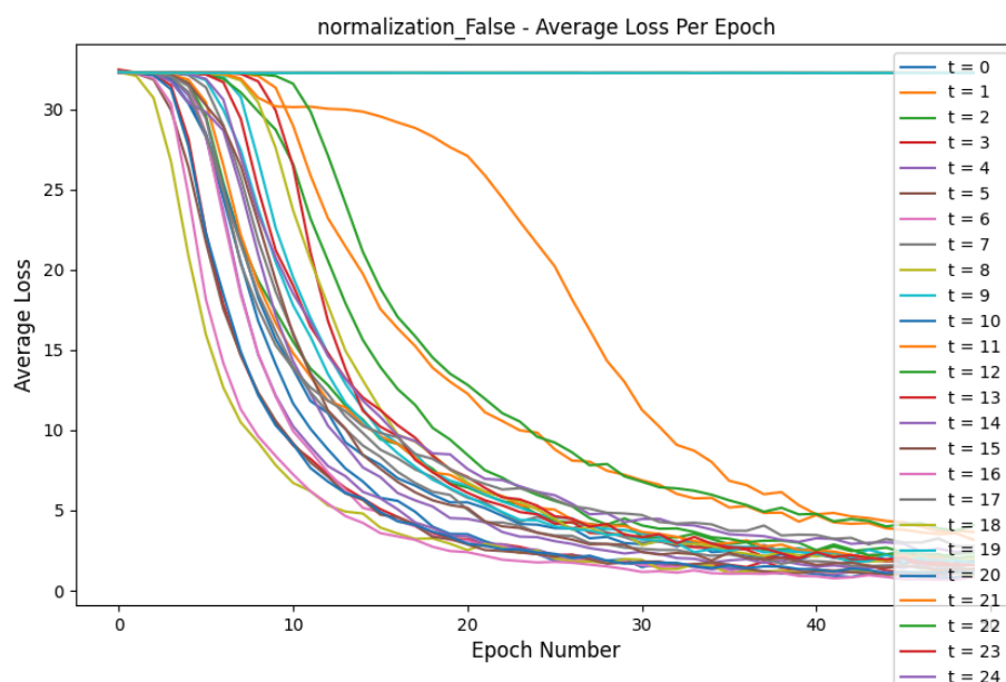
Figure 2: Loss Comparison for normalization_False experiment
