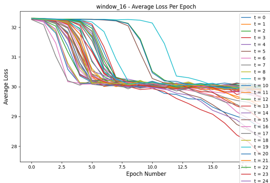
Figure 2: Loss Comparison for window_16 experiment
