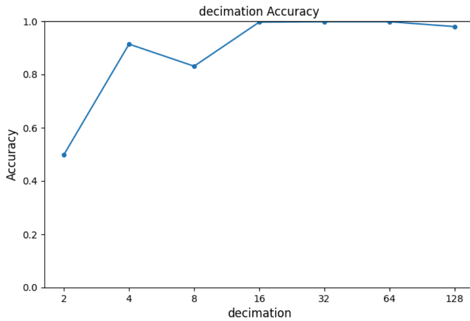
Figure 8: Accuracy Graph for decimation
