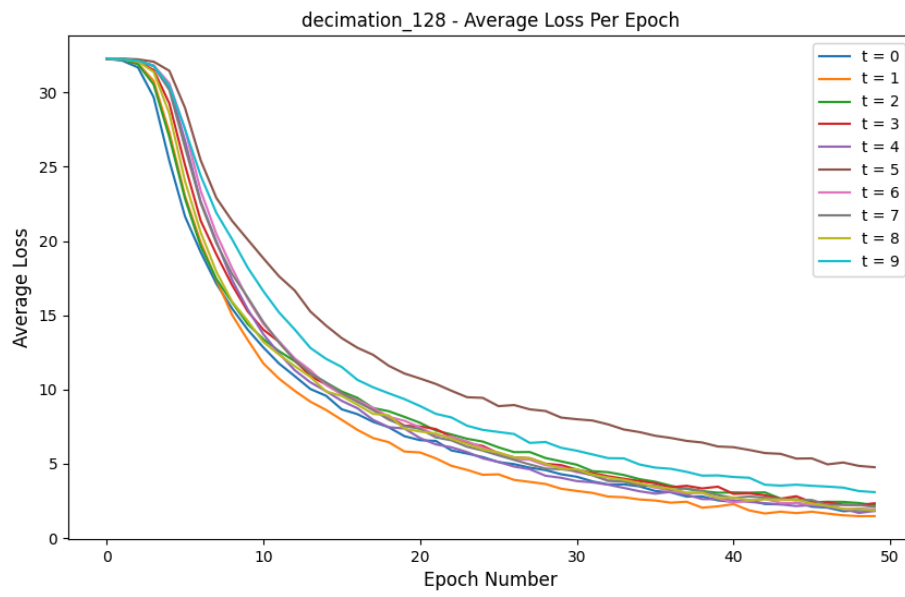
Figure 7: Loss Comparison for decimation_128 experiment
