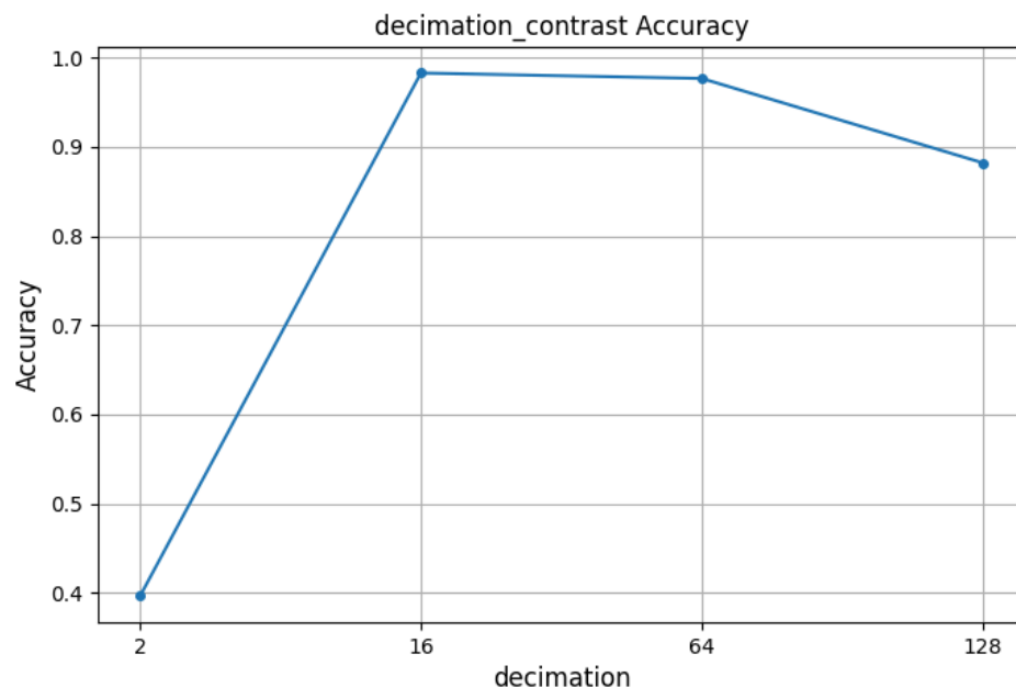
Figure 5: Accuracy Graph for decimation_contrast
