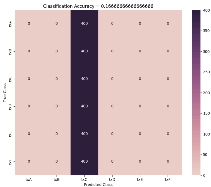
Figure 2: Confusion Matrix for windowed_random experiment
