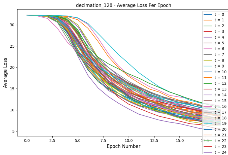
Figure 4: Loss Comparison for decimation_128 experiment
