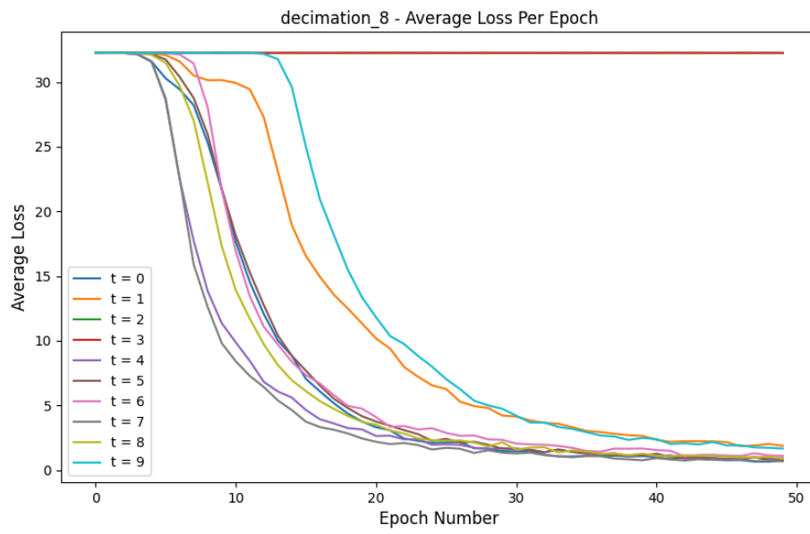
Figure 3: Loss Comparison for decimation_8 experiment
