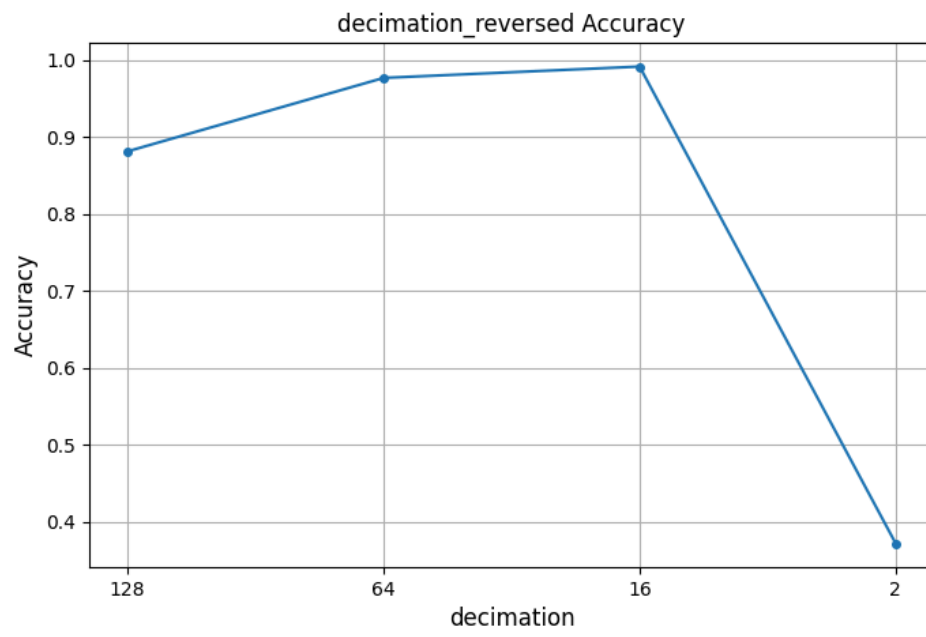
Figure 5: Accuracy Graph for decimation_reversed
