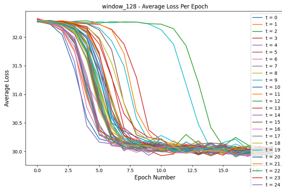
Figure 4: Loss Comparison for window_128 experiment
