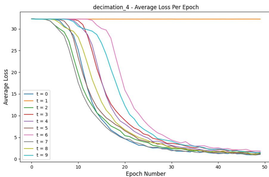
Figure 2: Loss Comparison for decimation_4 experiment
