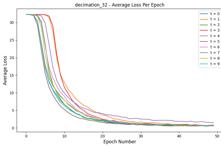
Figure 5: Loss Comparison for decimation_32 experiment
