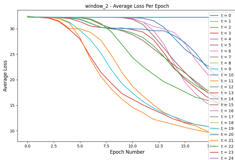
Figure 1: Loss Comparison for window_2 experiment
