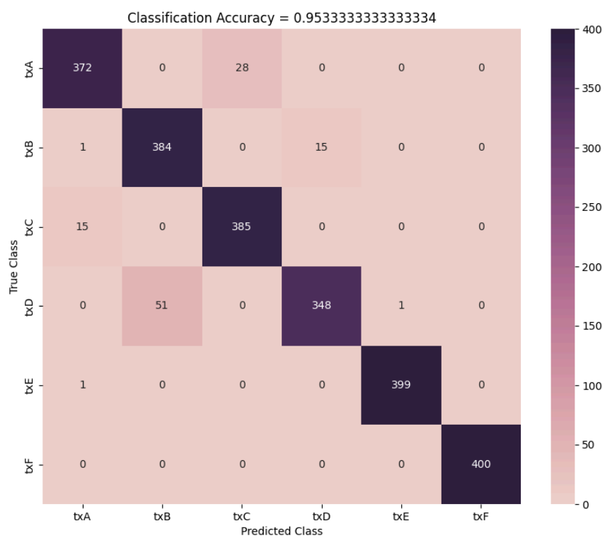
Figure 2: Confusion Matrix for room_fullwidth experiment
