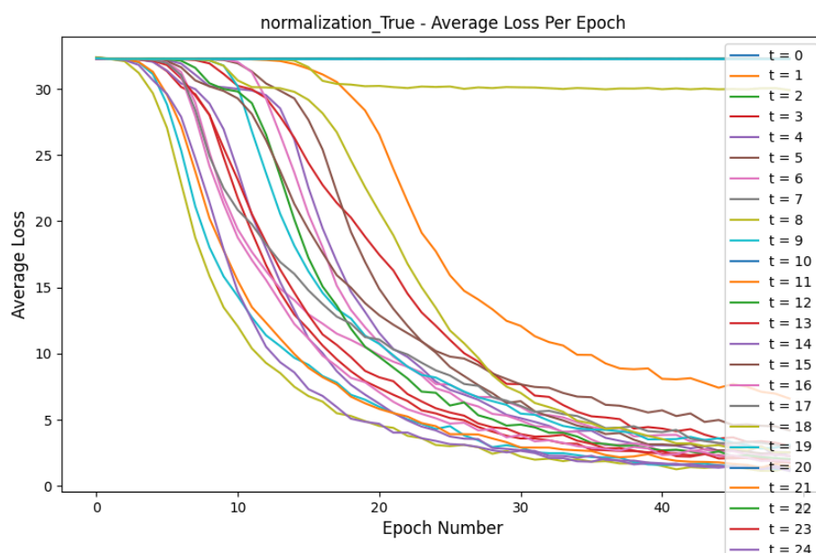
Figure 1: Loss Comparison for normalization_True experiment
