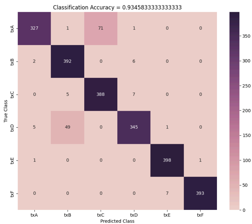
Figure 2: Confusion Matrix for room_main experiment
