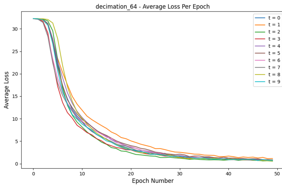
Figure 6: Loss Comparison for decimation_64 experiment
