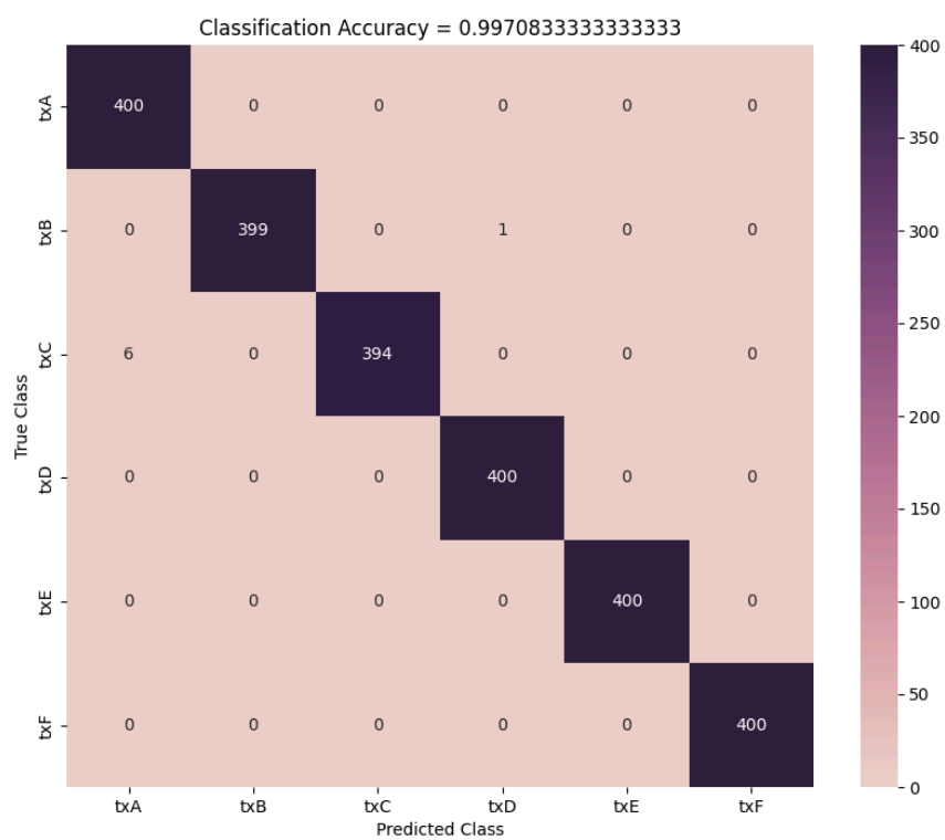
Figure 2: Confusion Matrix for wired_main experiment
