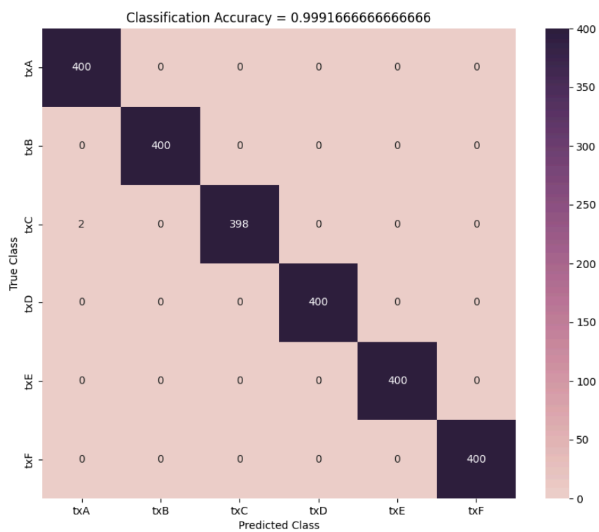
Figure 2: Confusion Matrix for wired_fullwidth experiment
