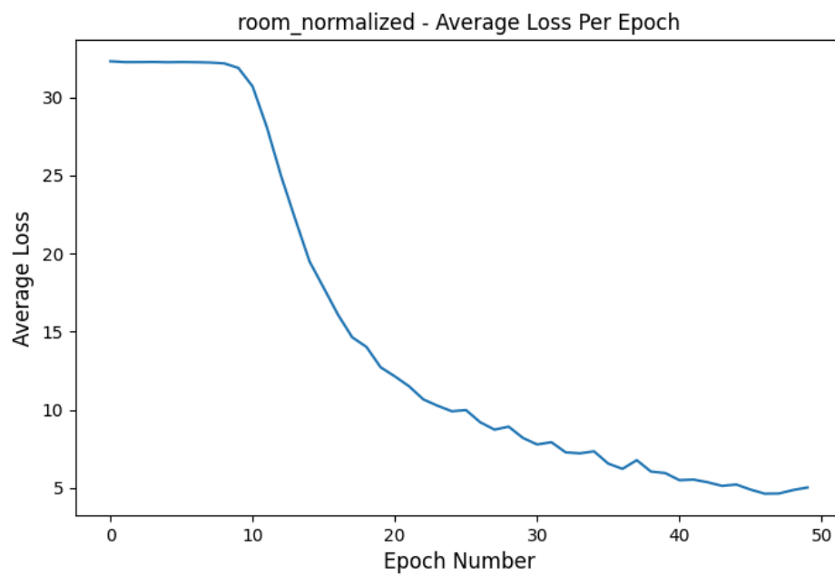
Figure 1: Loss Graph for room_normalized experiment
