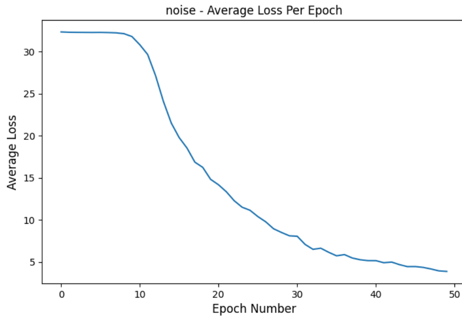
Figure 1: Loss Graph for noise experiment
