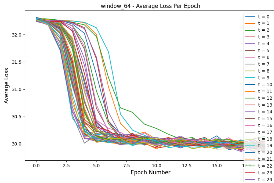
Figure 3: Loss Comparison for window_64 experiment
