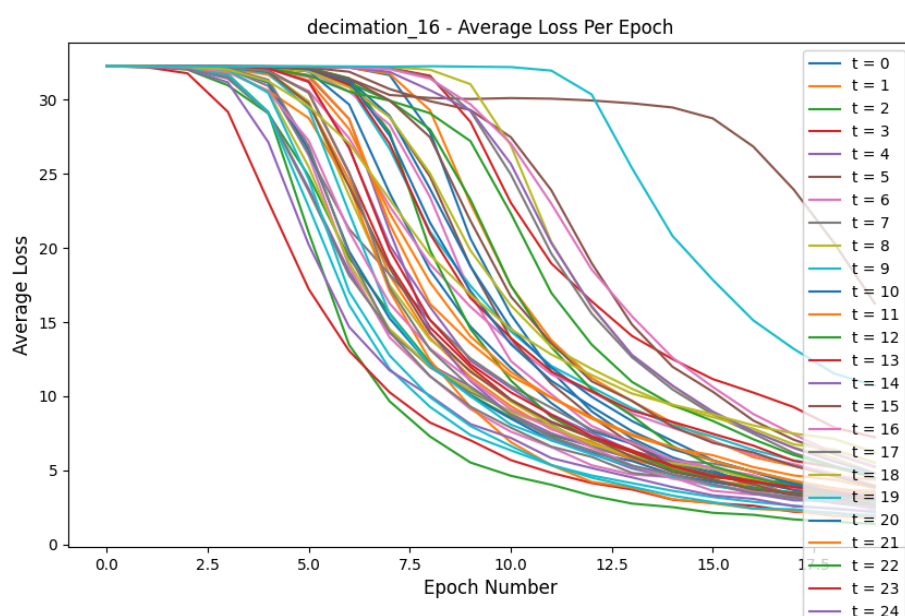
Figure 2: Loss Comparison for decimation_16 experiment
