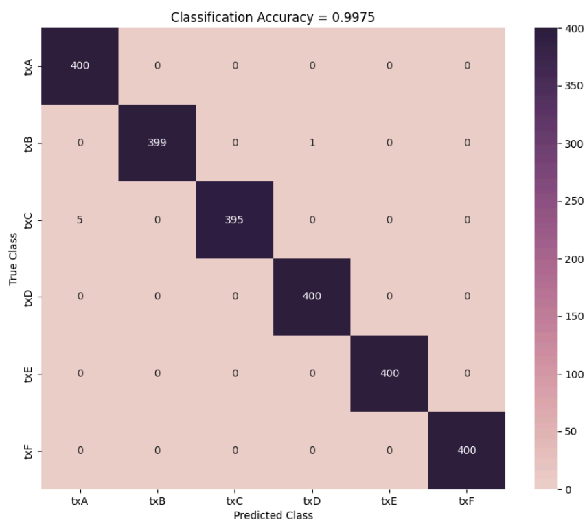
Figure 2: Confusion Matrix for wired_normalized experiment
