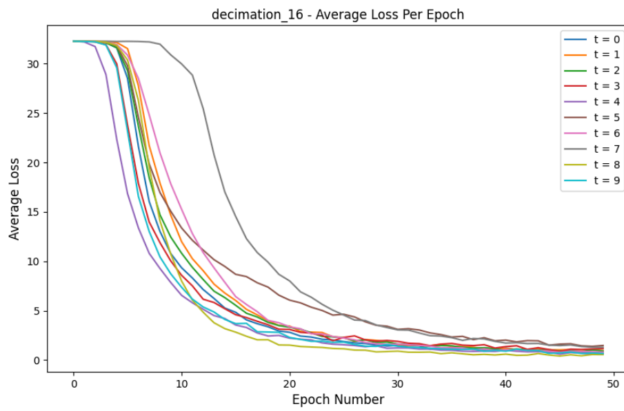
Figure 4: Loss Comparison for decimation_16 experiment
