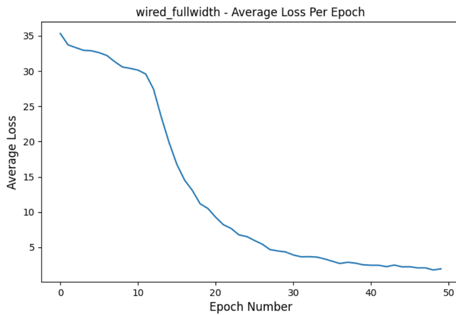
Figure 1: Loss Graph for wired_fullwidth experiment
