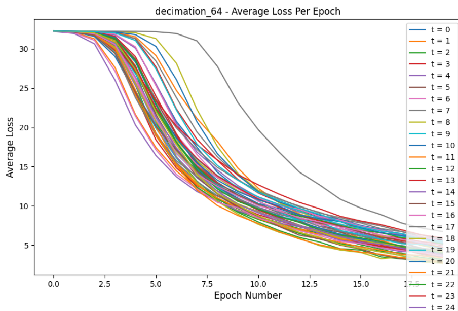
Figure 2: Loss Comparison for decimation_64 experiment
