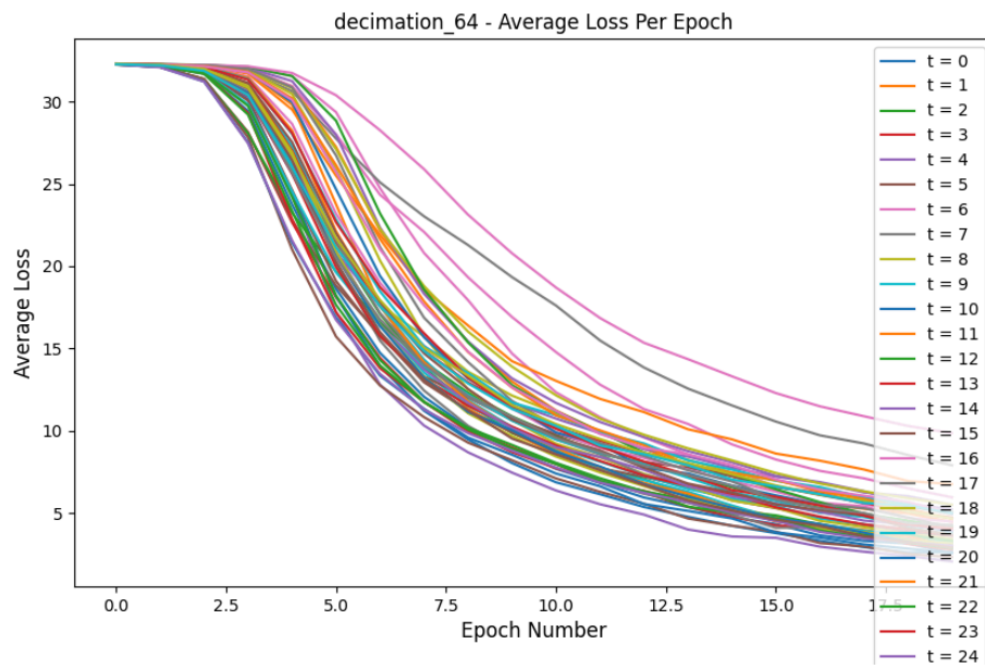
Figure 3: Loss Comparison for decimation_64 experiment
