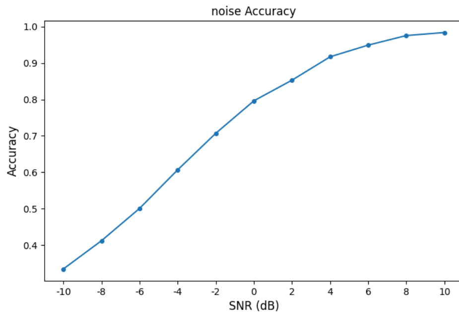
Figure 2: Accuracy Graph for noise
