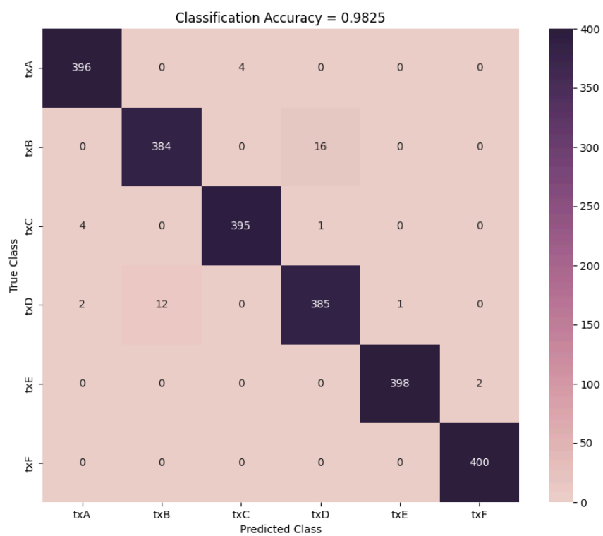
Figure 2: Confusion Matrix for room_normalized experiment
