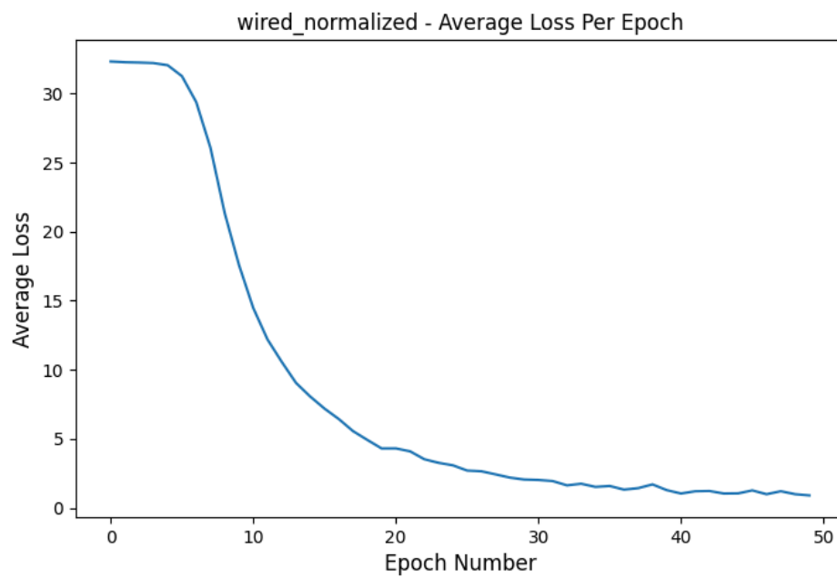
Figure 1: Loss Graph for wired_normalized experiment
