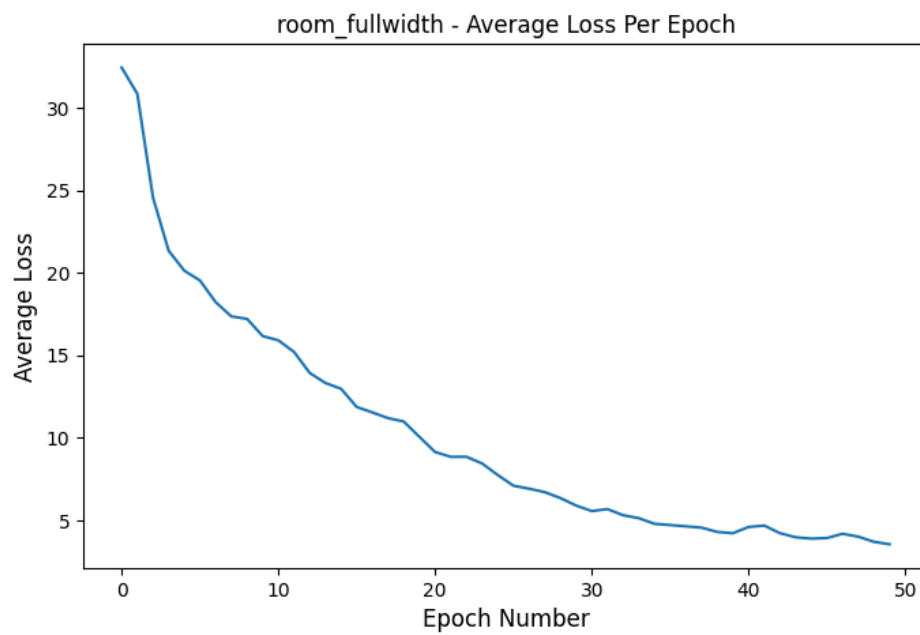
Figure 1: Loss Graph for room_fullwidth experiment
