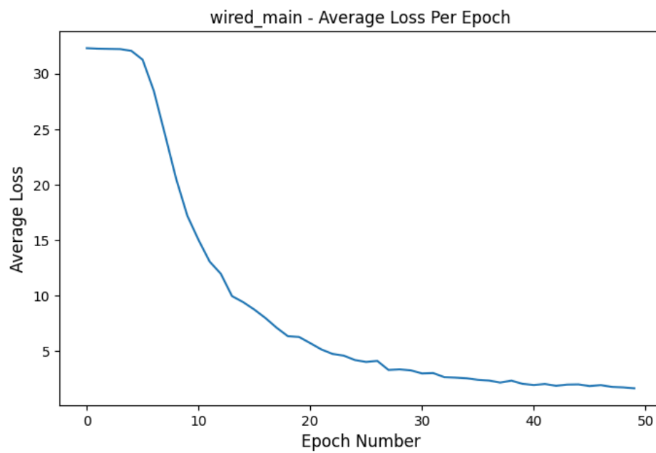
Figure 1: Loss Graph for wired_main experiment
