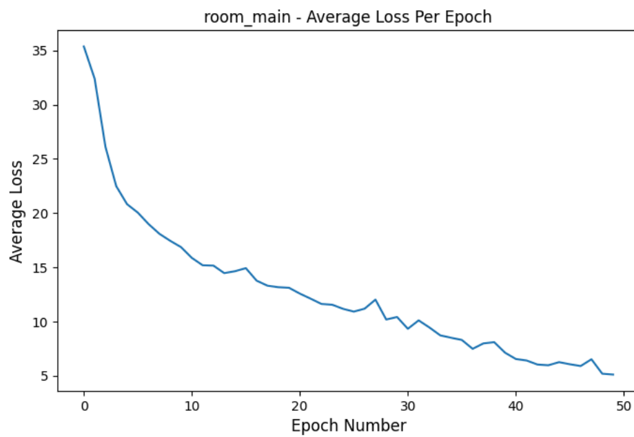
Figure 1: Loss Graph for room_main experiment
