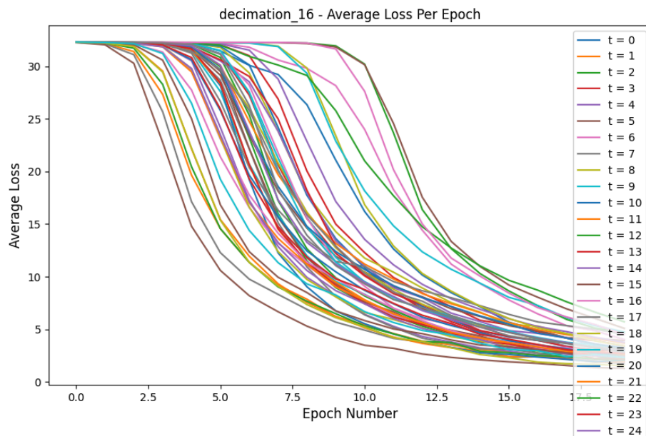
Figure 3: Loss Comparison for decimation_16 experiment
