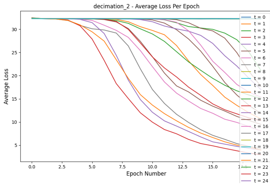
Figure 4: Loss Comparison for decimation_2 experiment
