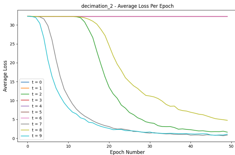
Figure 1: Loss Comparison for decimation_2 experiment
