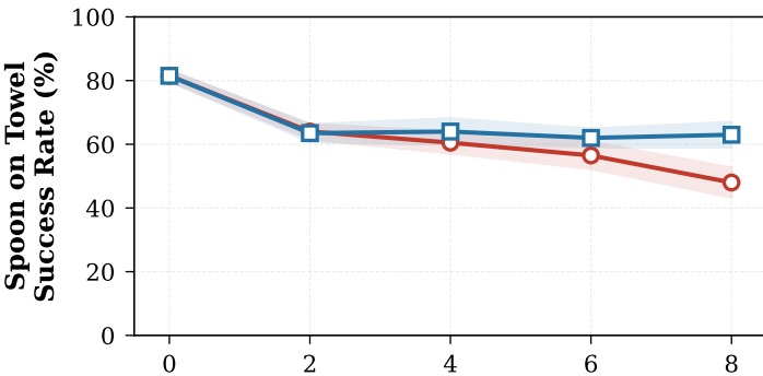
Semantic Distractors
