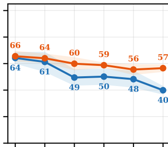
GR00T
