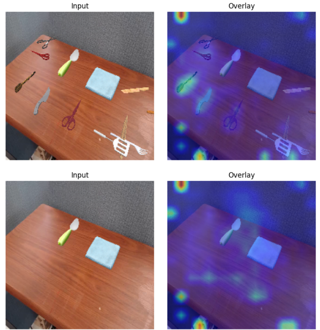
Fig. 2. Qualitative illustration of the attention-repair hypothesis (policy input and attention overlay). (Top) Under clutter, the baseline policy’s attention is dispersed across distractors rather than the spoon. (Bottom) With CGVD, attention concentrates more on the target region. Maps are produced by the evaluation harness’s attention-capture instrument: hooks on every self-attention layer of \pi_0 ’s PaliGemma backbone recompute \text{softmax}(QK^\top/\sqrt{d}) ; attention from the final query token onto the 256 SigLIP visual tokens ( 16 \times 16 grid) is averaged over all layers and heads, captured at the first inference step of an episode (baseline: raw frame; CGVD: distilled frame). Because deleting a distractor’s pixels necessarily deletes attention on those pixels, this figure illustrates the hypothesis but cannot by itself discriminate it from alternatives (§IV-B).
