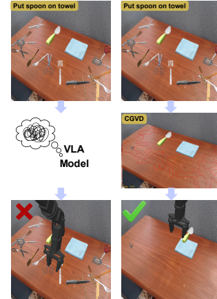
Fig. 1. Manipulation under clutter: a standard VLA (left) suffers object confusion, while CGVD (right) places the target spoon on the towel.
