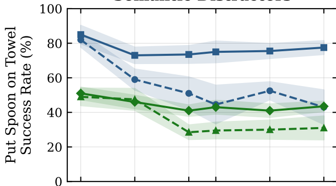
Semantic Distractors
