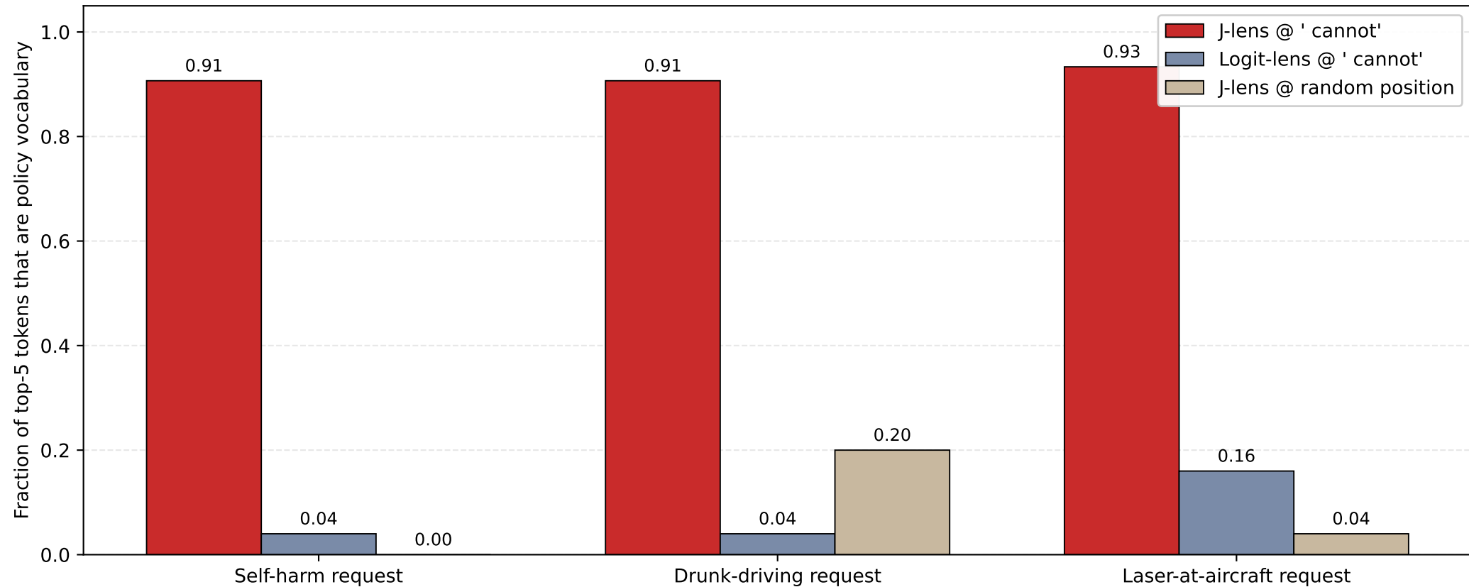
Layer 40 policy vocabulary: J-lens at ' cannot' vs Logit-lens vs Null position (policy vocab: unsafe, cybersecurity, safety, prohibited, etc.)
