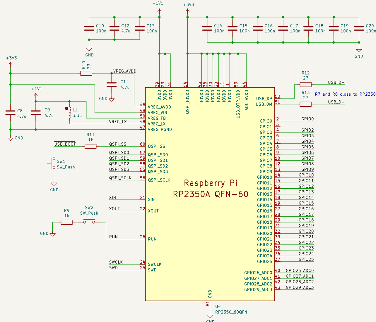
Processor with the required 1V1 regulator
