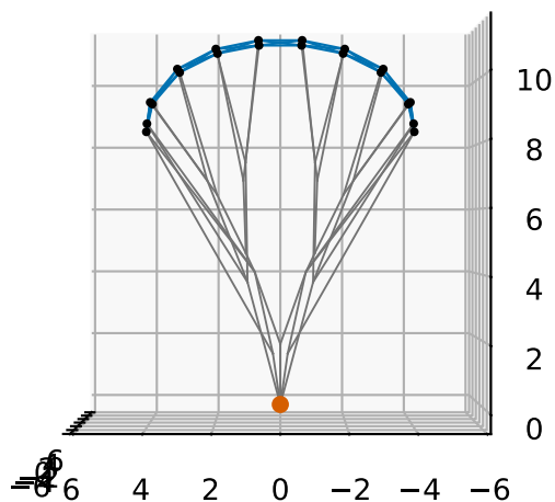
FEM before stretching
