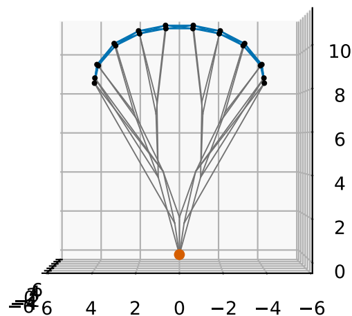
FEM after stretching
